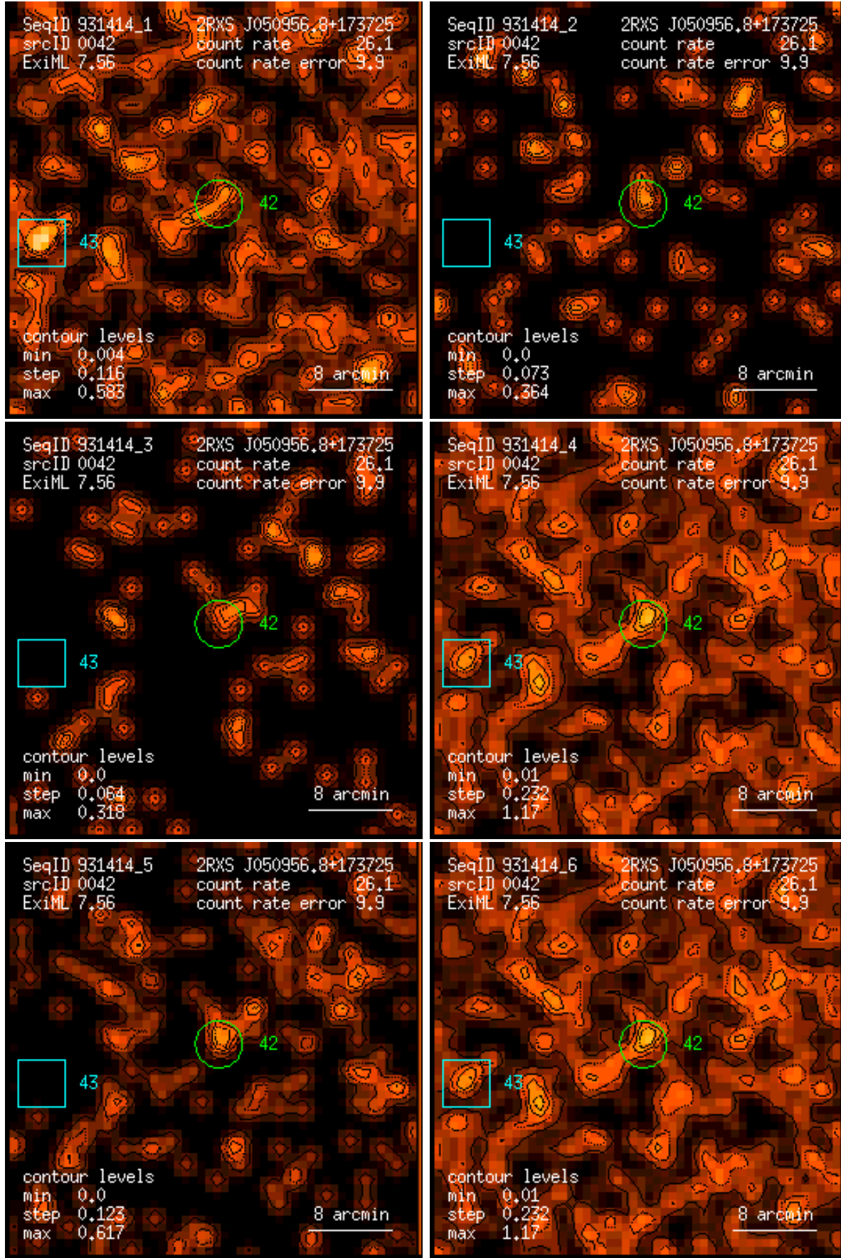
Figure 42: RASS 931414: detection 0042: band rate images, Gaussian filter: (1) PSPC channels 11 – 41, (2) 52 – 90, (3) 91 – 201, (4) 11 – 235, (5) 52 – 201, (6) 11 – 201. Broad band rates in counts/ks. Band rate contour levels in counts/ks/arcmin 2 .
