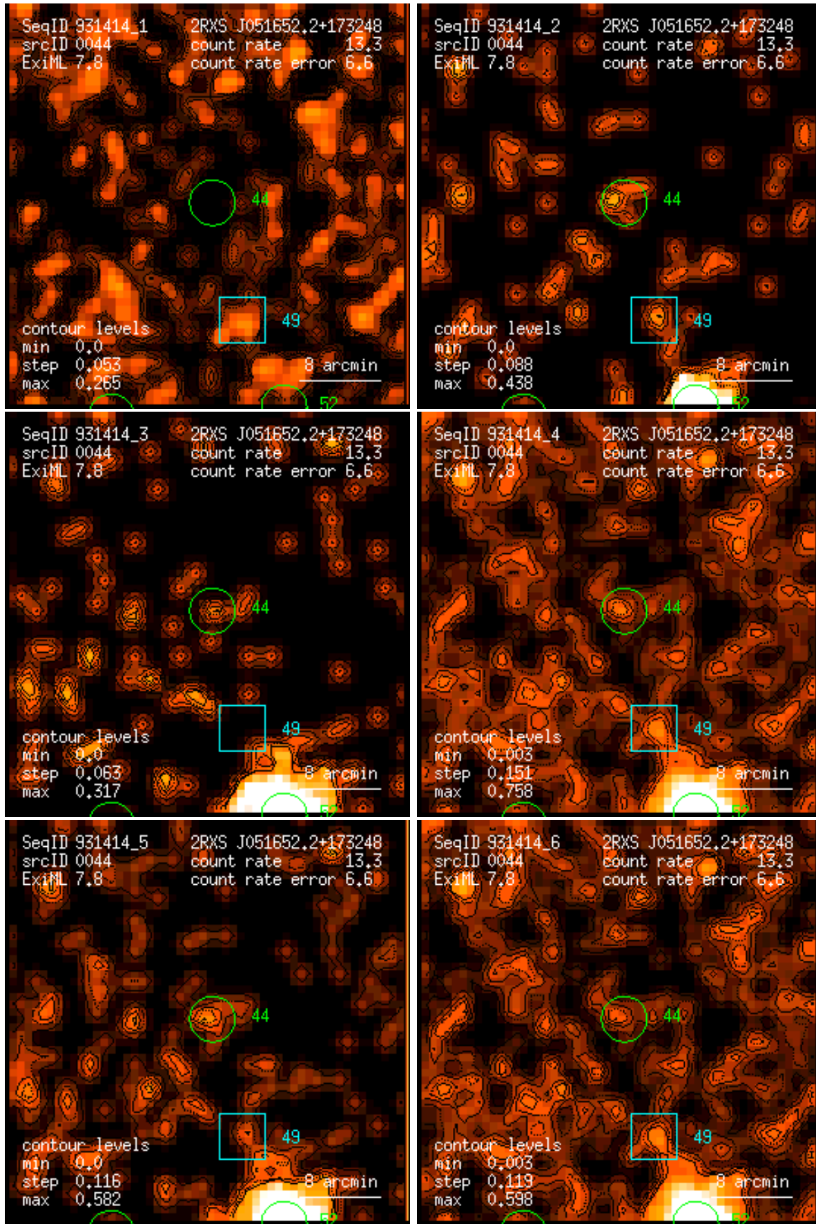
Figure 44: RASS 931414: detection 0044: band rate images, Gaussian filter: (1) PSPC channels 11 – 41, (2) 52 – 90, (3) 91 – 201, (4) 11 – 235, (5) 52 – 201, (6) 11 – 201. Broad band rates in counts/ks. Band rate contour levels in counts/ks/arcmin 2 .
