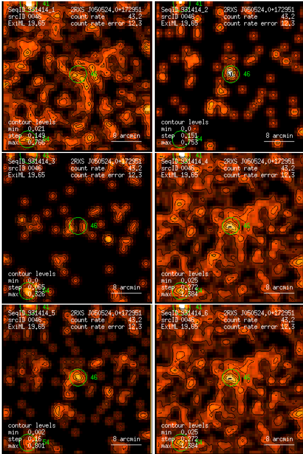
Figure 46: RASS 931414: detection 0046: band rate images, Gaussian filter: (1) PSPC channels 11 – 41, (2) 52 – 90, (3) 91 – 201, (4) 11 – 235, (5) 52 – 201, (6) 11 – 201. Broad band rates in counts/ks. Band rate contour levels in counts/ks/arcmin 2 .
