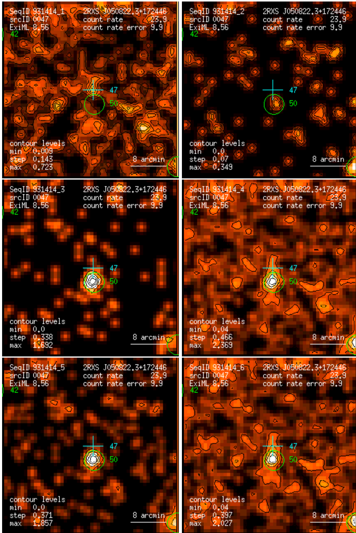
Figure 47: RASS 931414: detection 0047: band rate images, Gaussian filter: (1) PSPC channels 11 – 41, (2) 52 – 90, (3) 91 – 201, (4) 11 – 235, (5) 52 – 201, (6) 11 – 201. Broad band rates in counts/ks. Band rate contour levels in counts/ks/arcmin 2 .
