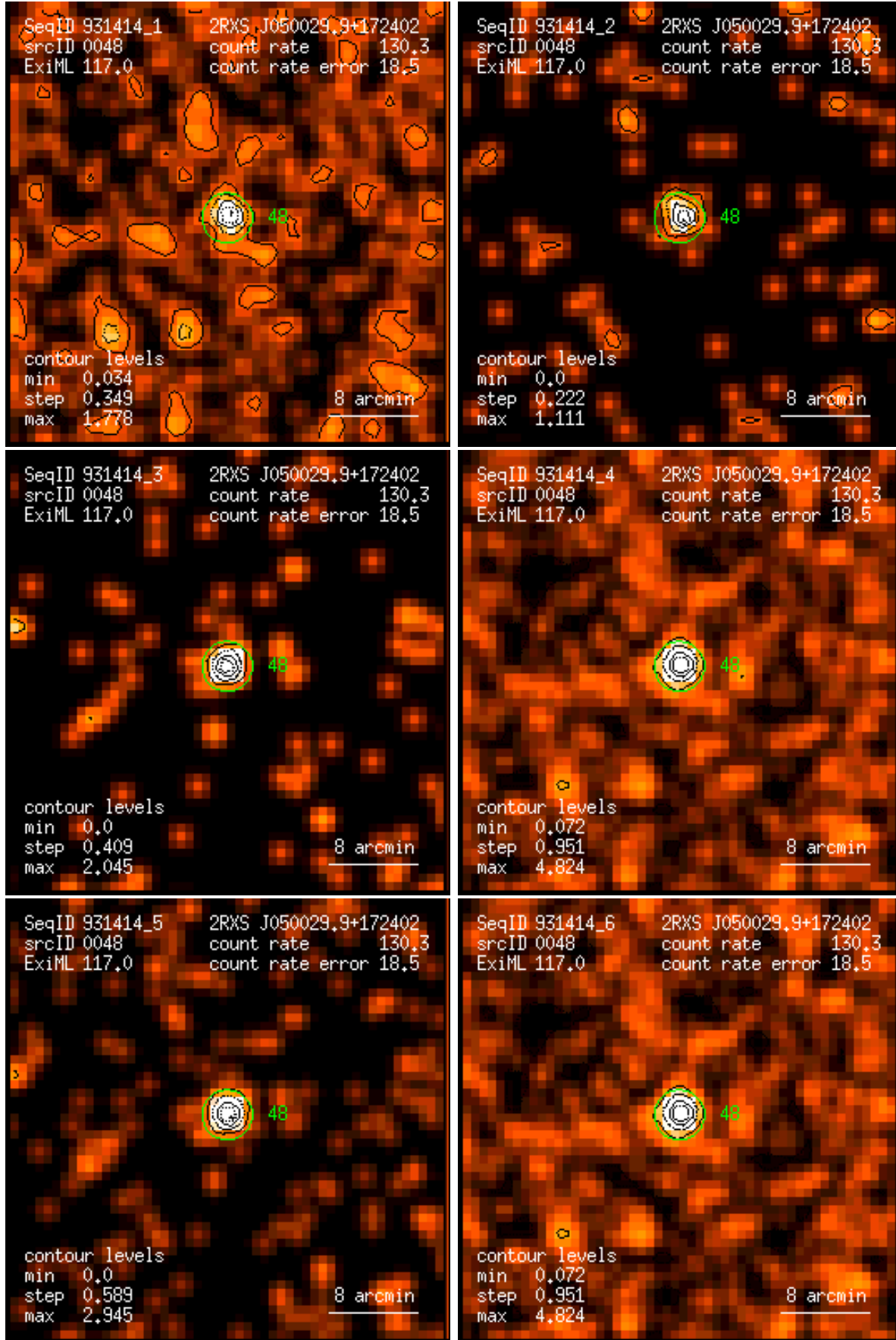
Figure 48: RASS 931414: detection 0048: band rate images, Gaussian filter: (1) PSPC channels 11 – 41, (2) 52 – 90, (3) 91 – 201, (4) 11 – 235, (5) 52 – 201, (6) 11 – 201. Broad band rates in counts/ks. Band rate contour levels in counts/ks/arcmin 2 .
