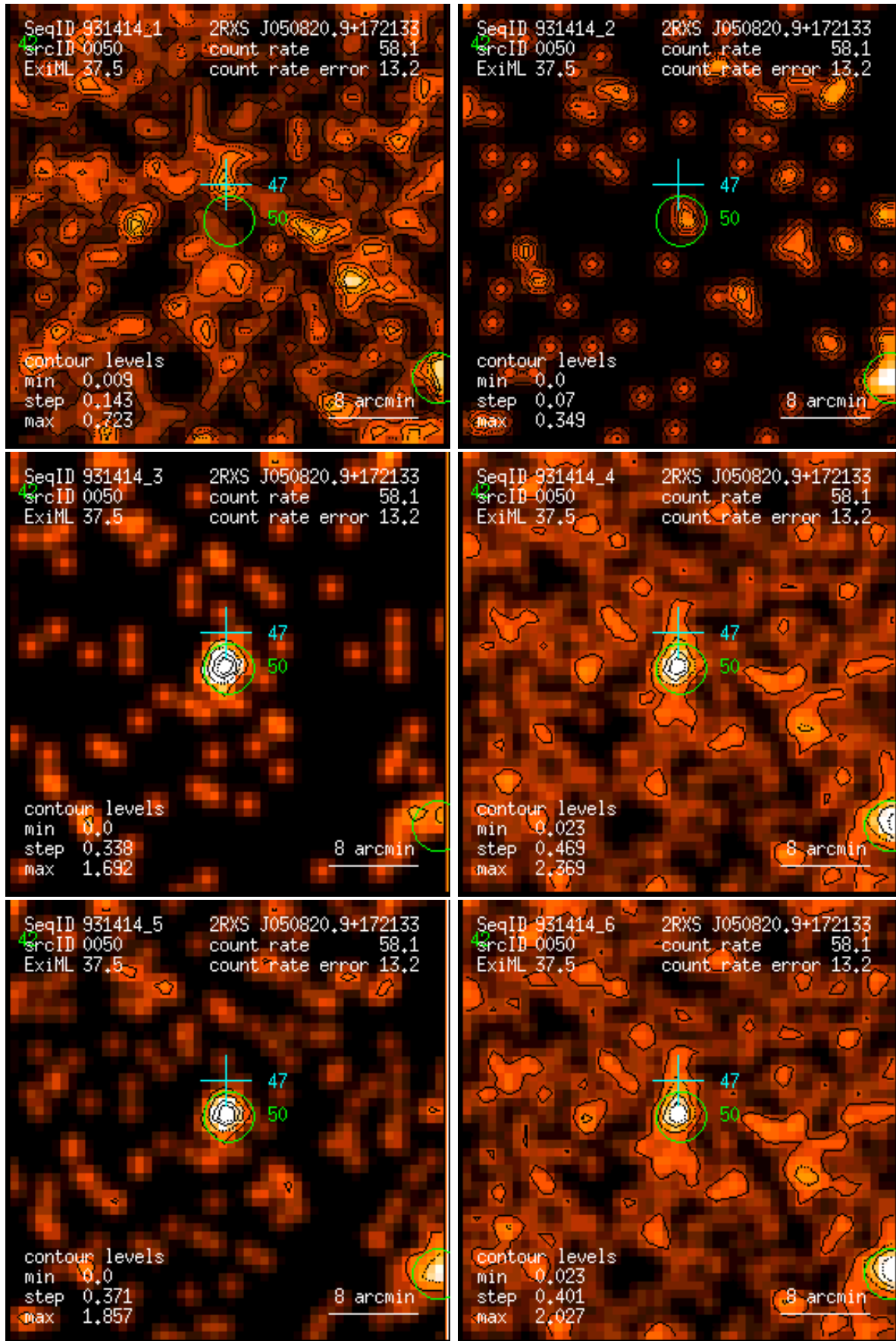
Figure 50: RASS 931414: detection 0050: band rate images, Gaussian filter: (1) PSPC channels 11 – 41, (2) 52 – 90, (3) 91 – 201, (4) 11 – 235, (5) 52 – 201, (6) 11 – 201. Broad band rates in counts/ks. Band rate contour levels in counts/ks/arcmin 2 .
