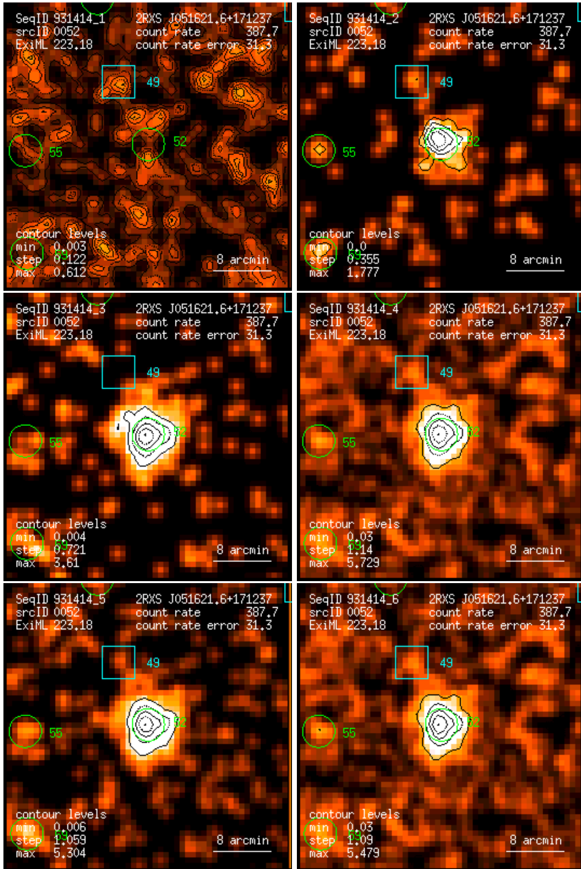
Figure 52: RASS 931414: detection 0052: band rate images, Gaussian filter: (1) PSPC channels 11 – 41, (2) 52 – 90, (3) 91 – 201, (4) 11 – 235, (5) 52 – 201, (6) 11 – 201. Broad band rates in counts/ks. Band rate contour levels in counts/ks/arcmin 2 .
