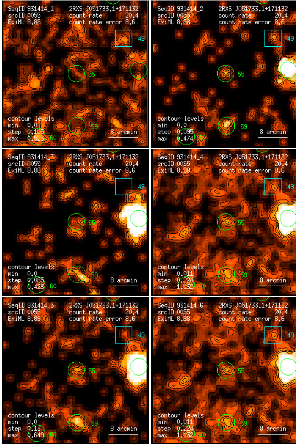
Figure 55: RASS 931414: detection 0055: band rate images, Gaussian filter: (1) PSPC channels 11 – 41, (2) 52 – 90, (3) 91 – 201, (4) 11 – 235, (5) 52 – 201, (6) 11 – 201. Broad band rates in counts/ks. Band rate contour levels in counts/ks/arcmin 2 .
