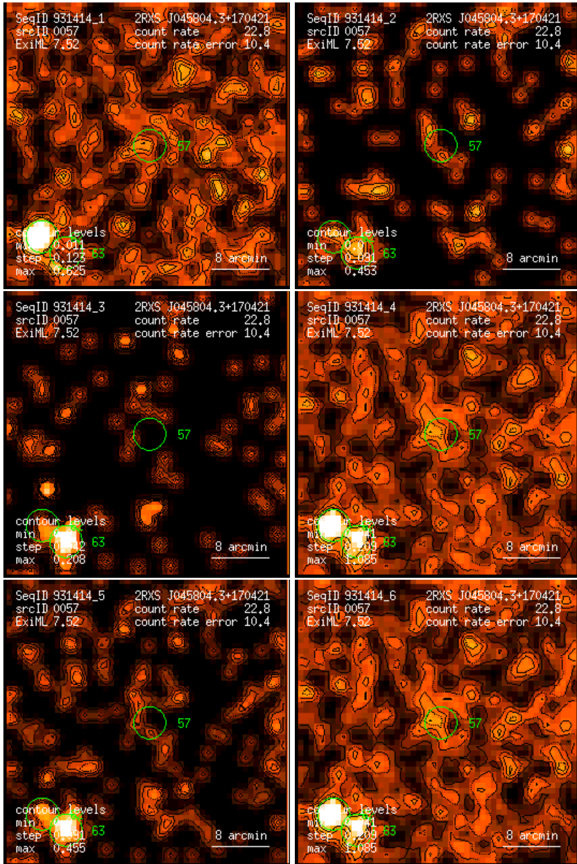
Figure 57: RASS 931414: detection 0057: band rate images, Gaussian filter: (1) PSPC channels 11 – 41, (2) 52 – 90, (3) 91 – 201, (4) 11 – 235, (5) 52 – 201, (6) 11 – 201. Broad band rates in counts/ks. Band rate contour levels in counts/ks/arcmin 2 .
