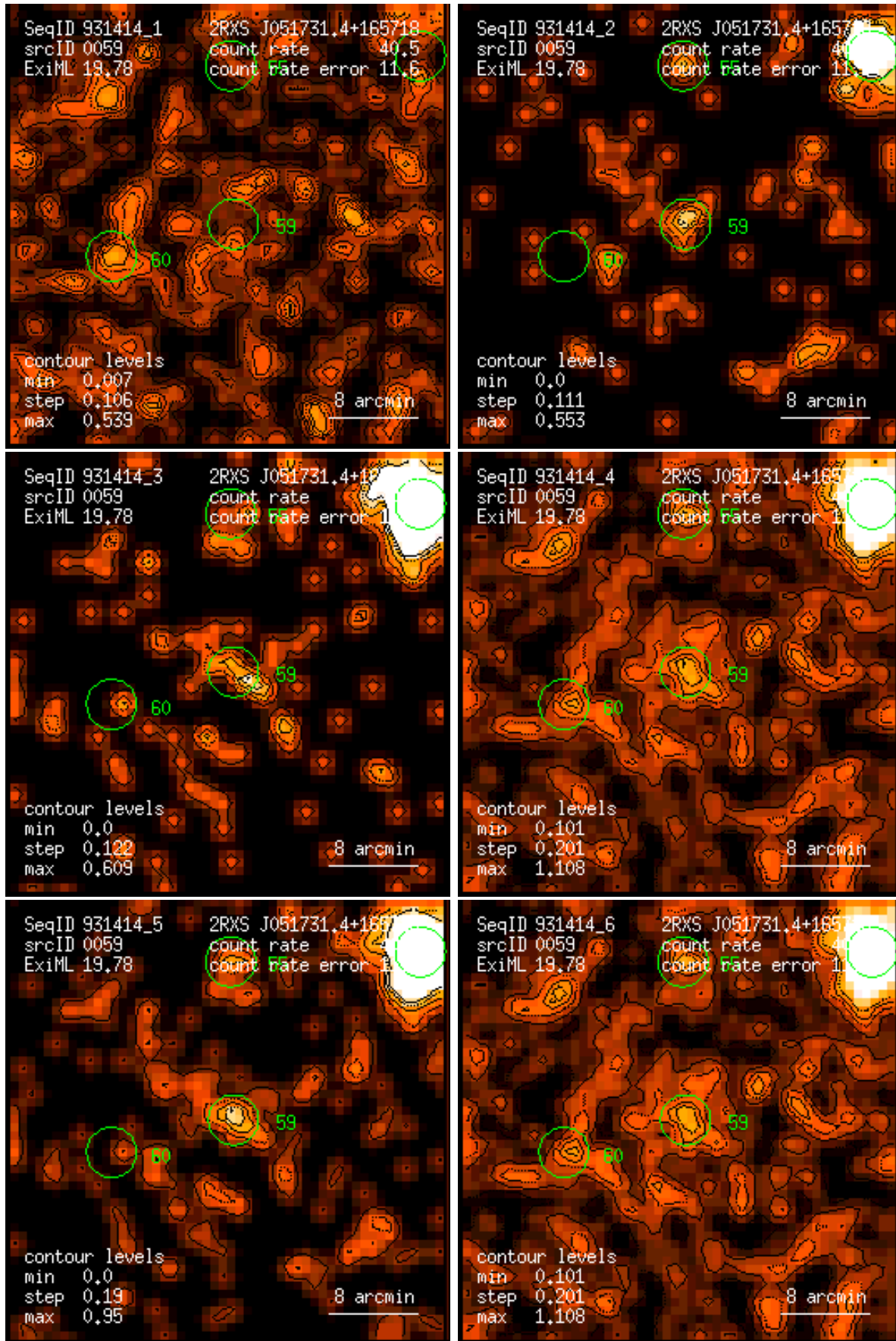
Figure 59: RASS 931414: detection 0059: band rate images, Gaussian filter: (1) PSPC channels 11 – 41, (2) 52 – 90, (3) 91 – 201, (4) 11 – 235, (5) 52 – 201, (6) 11 – 201. Broad band rates in counts/ks. Band rate contour levels in counts/ks/arcmin 2 .
