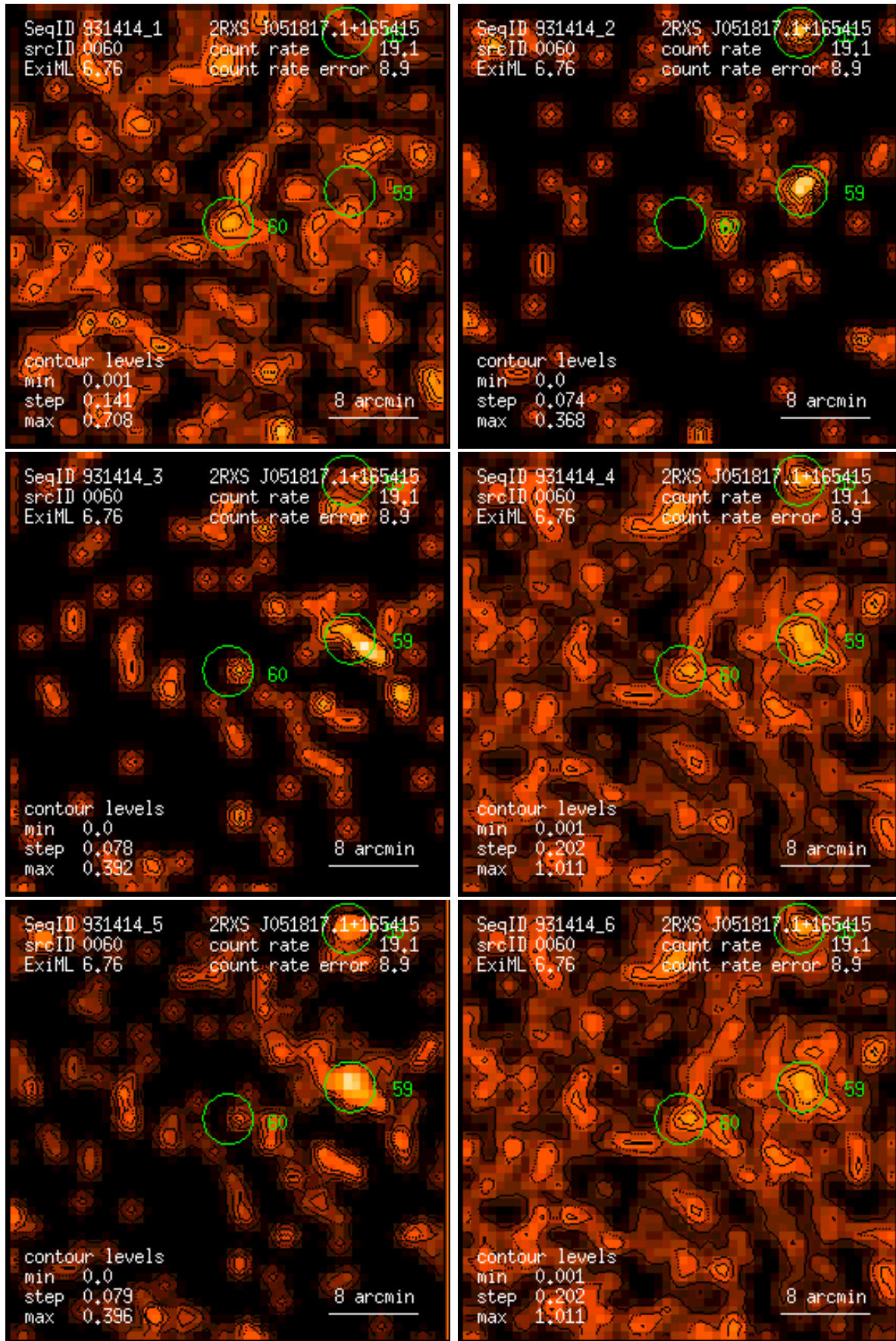
Figure 60: RASS 931414: detection 0060: band rate images, Gaussian filter: (1) PSPC channels 11 – 41, (2) 52 – 90, (3) 91 – 201, (4) 11 – 235, (5) 52 – 201, (6) 11 – 201. Broad band rates in counts/ks. Band rate contour levels in counts/ks/arcmin 2 .
