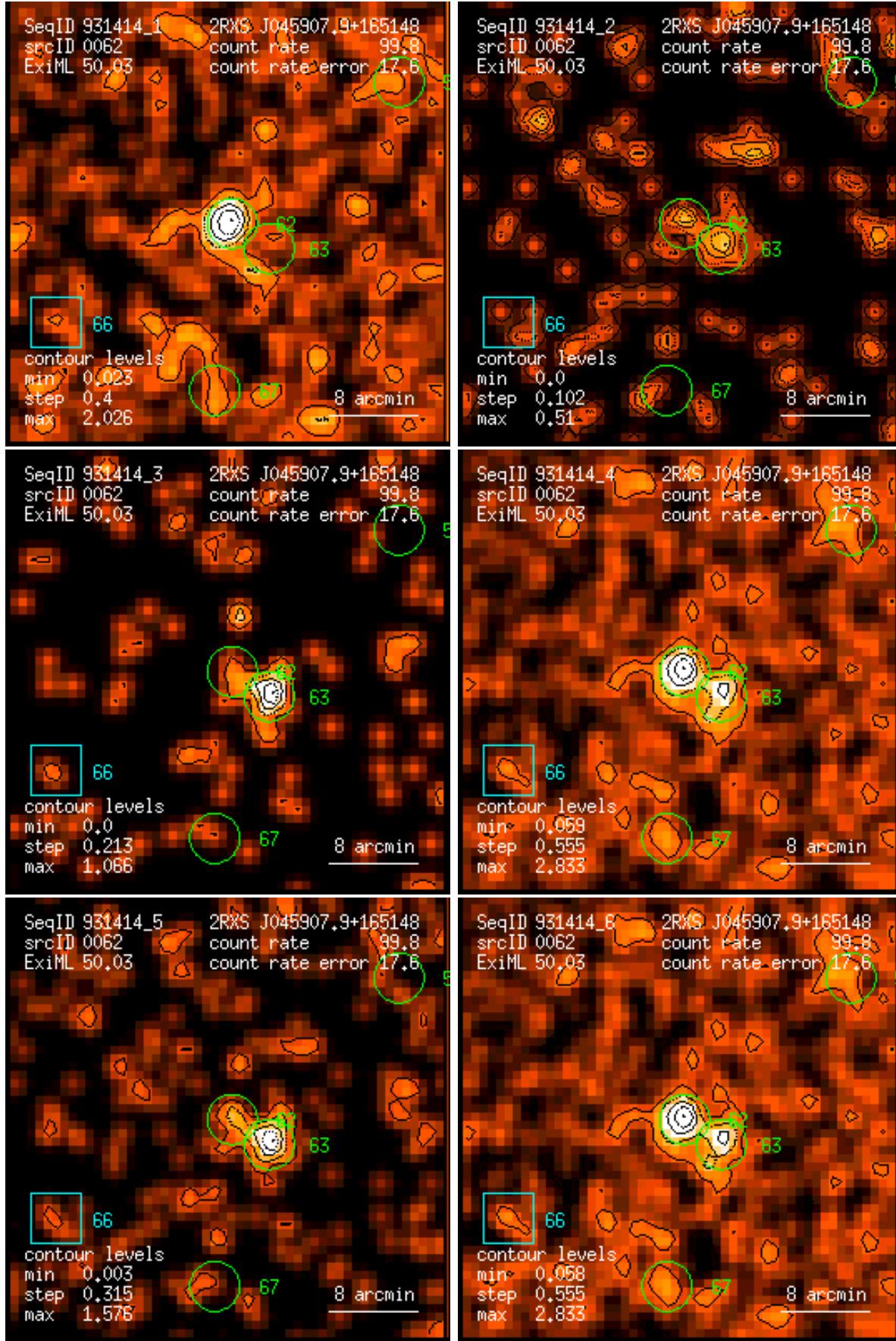
Figure 62: RASS 931414: detection 0062: band rate images, Gaussian filter: (1) PSPC channels 11 – 41, (2) 52 – 90, (3) 91 – 201, (4) 11 – 235, (5) 52 – 201, (6) 11 – 201. Broad band rates in counts/ks. Band rate contour levels in counts/ks/arcmin 2 .
