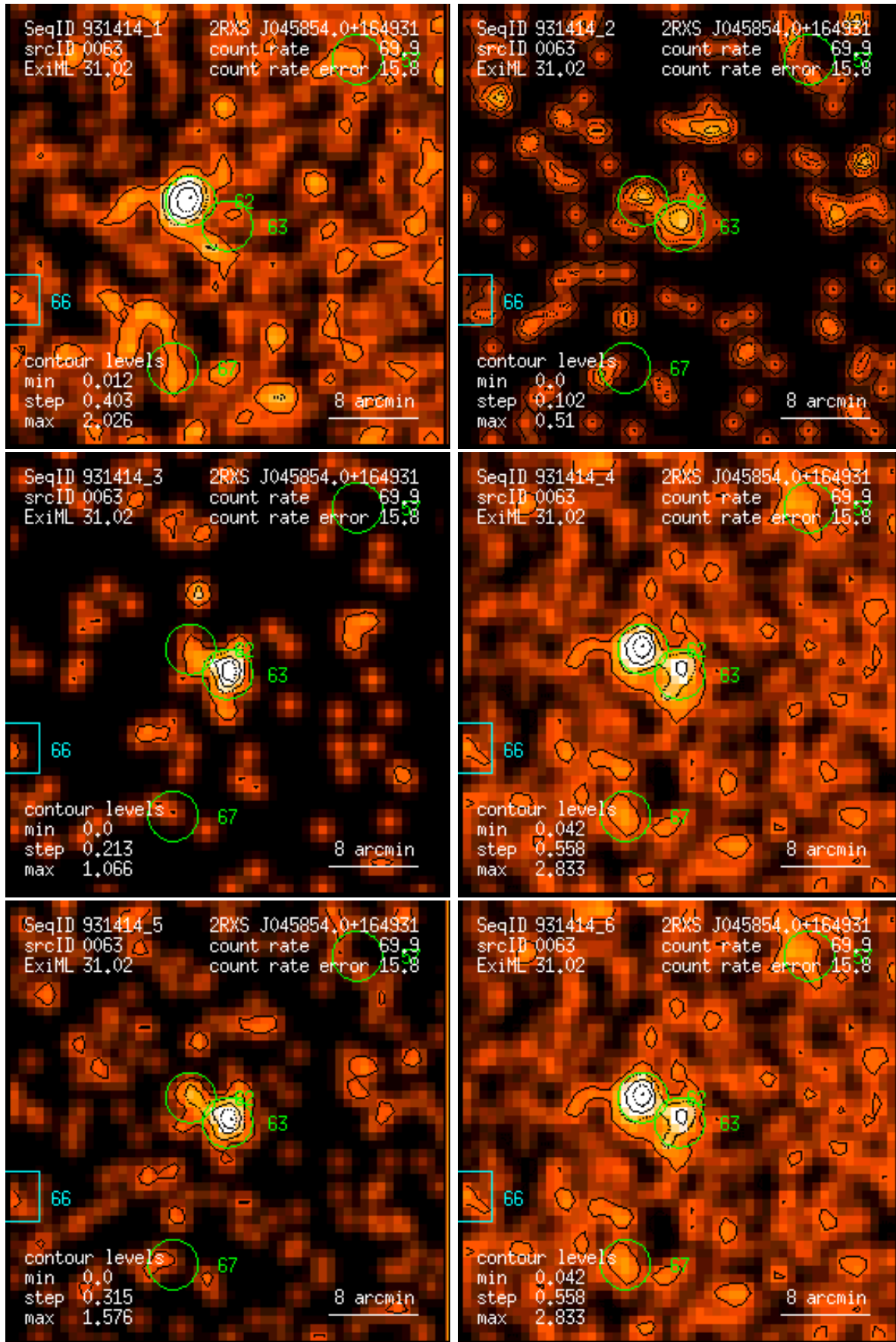
Figure 63: RASS 931414: detection 0063: band rate images, Gaussian filter: (1) PSPC channels 11 – 41, (2) 52 – 90, (3) 91 – 201, (4) 11 – 235, (5) 52 – 201, (6) 11 – 201. Broad band rates in counts/ks. Band rate contour levels in counts/ks/arcmin 2 .
