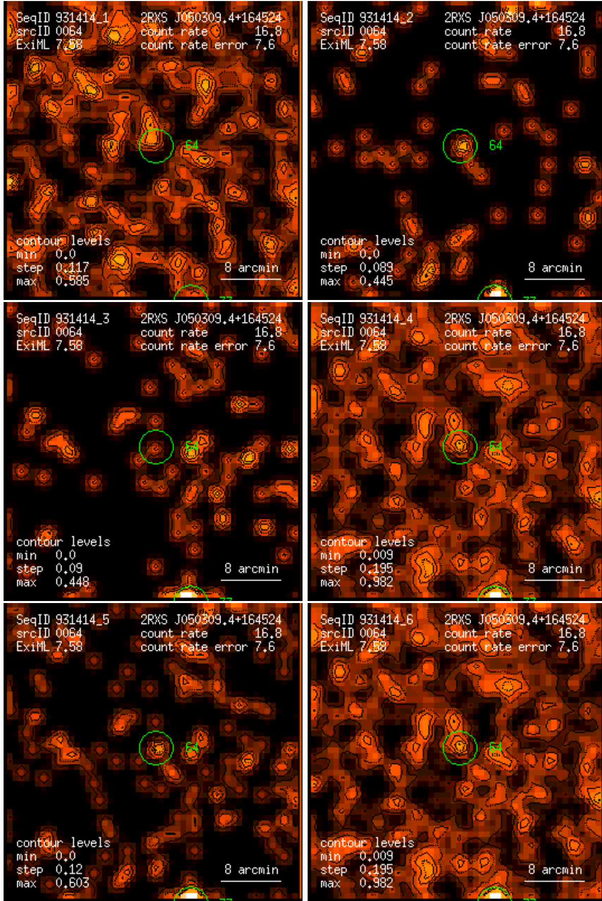
Figure 64: RASS 931414: detection 0064: band rate images, Gaussian filter: (1) PSPC channels 11 – 41, (2) 52 – 90, (3) 91 – 201, (4) 11 – 235, (5) 52 – 201, (6) 11 – 201. Broad band rates in counts/ks. Band rate contour levels in counts/ks/arcmin 2 .
