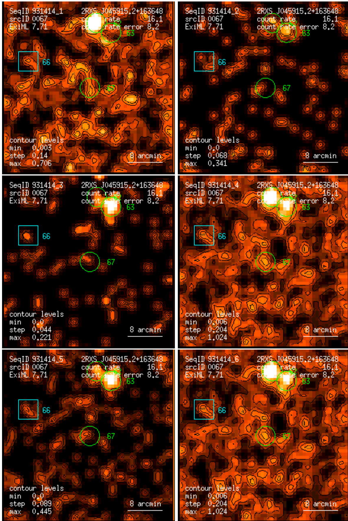
Figure 67: RASS 931414: detection 0067: band rate images, Gaussian filter: (1) PSPC channels 11 – 41, (2) 52 – 90, (3) 91 – 201, (4) 11 – 235, (5) 52 – 201, (6) 11 – 201. Broad band rates in counts/ks. Band rate contour levels in counts/ks/arcmin 2 .
