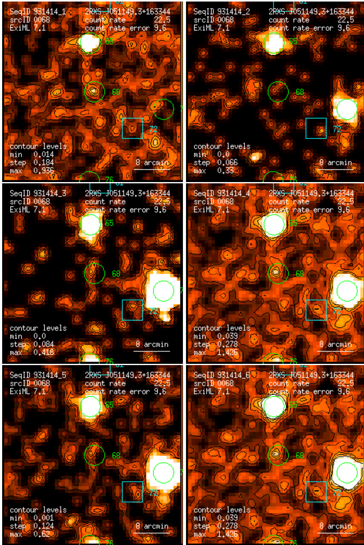
Figure 68: RASS 931414: detection 0068: band rate images, Gaussian filter: (1) PSPC channels 11 – 41, (2) 52 – 90, (3) 91 – 201, (4) 11 – 235, (5) 52 – 201, (6) 11 – 201. Broad band rates in counts/ks. Band rate contour levels in counts/ks/arcmin 2 .
