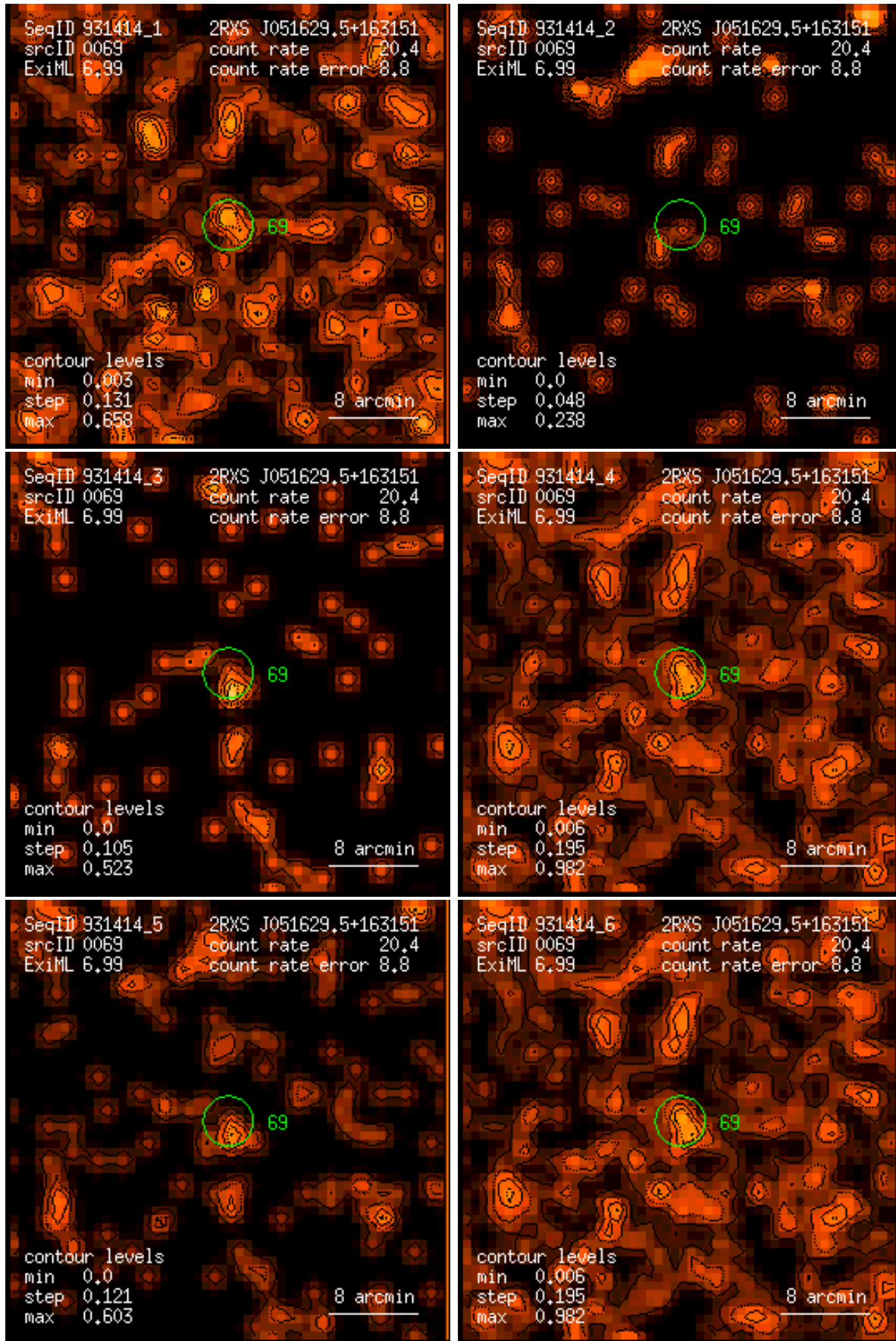
Figure 69: RASS 931414: detection 0069: band rate images, Gaussian filter: (1) PSPC channels 11 – 41, (2) 52 – 90, (3) 91 – 201, (4) 11 – 235, (5) 52 – 201, (6) 11 – 201. Broad band rates in counts/ks. Band rate contour levels in counts/ks/arcmin 2 .
