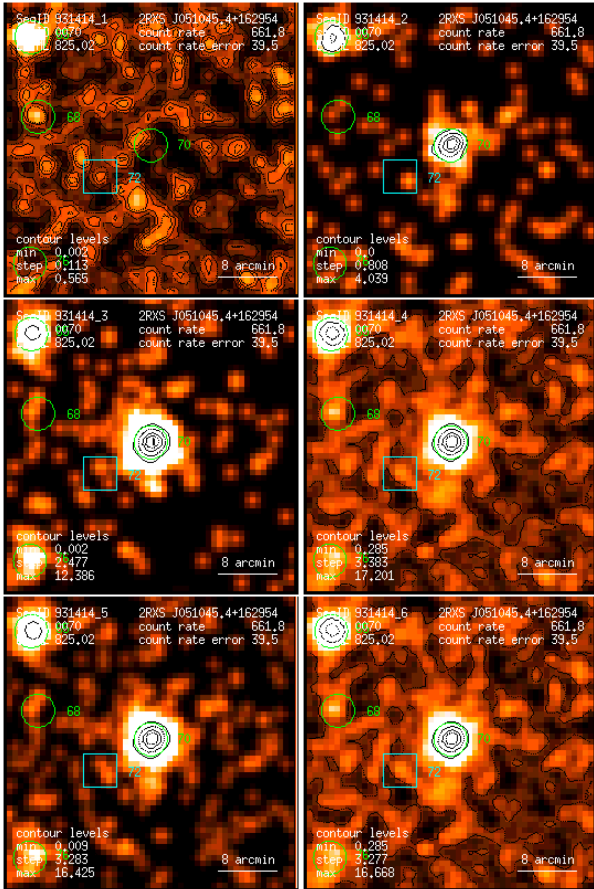
Figure 70: RASS 931414: detection 0070: band rate images, Gaussian filter: (1) PSPC channels 11 – 41, (2) 52 – 90, (3) 91 – 201, (4) 11 – 235, (5) 52 – 201, (6) 11 – 201. Broad band rates in counts/ks. Band rate contour levels in counts/ks/arcmin 2 .
