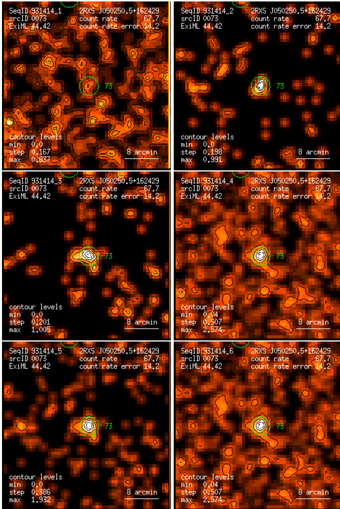
Figure 73: RASS 931414: detection 0073: band rate images, Gaussian filter: (1) PSPC channels 11 – 41, (2) 52 – 90, (3) 91 – 201, (4) 11 – 235, (5) 52 – 201, (6) 11 – 201. Broad band rates in counts/ks. Band rate contour levels in counts/ks/arcmin 2 .
