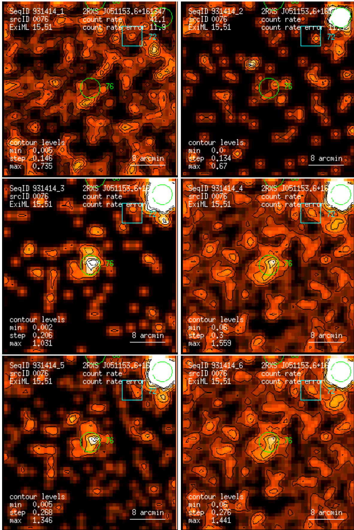
Figure 76: RASS 931414: detection 0076: band rate images, Gaussian filter: (1) PSPC channels 11 – 41, (2) 52 – 90, (3) 91 – 201, (4) 11 – 235, (5) 52 – 201, (6) 11 – 201. Broad band rates in counts/ks. Band rate contour levels in counts/ks/arcmin 2 .
