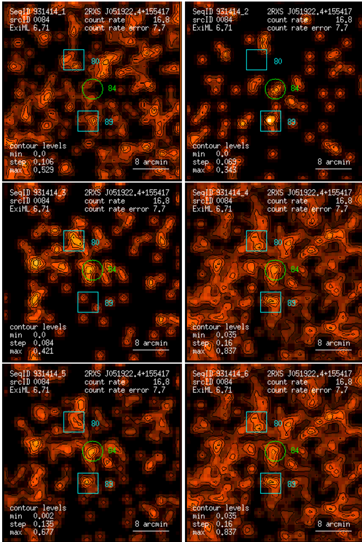
Figure 84: RASS 931414: detection 0084: band rate images, Gaussian filter: (1) PSPC channels 11 – 41, (2) 52 – 90, (3) 91 – 201, (4) 11 – 235, (5) 52 – 201, (6) 11 – 201. Broad band rates in counts/ks. Band rate contour levels in counts/ks/arcmin 2 .
