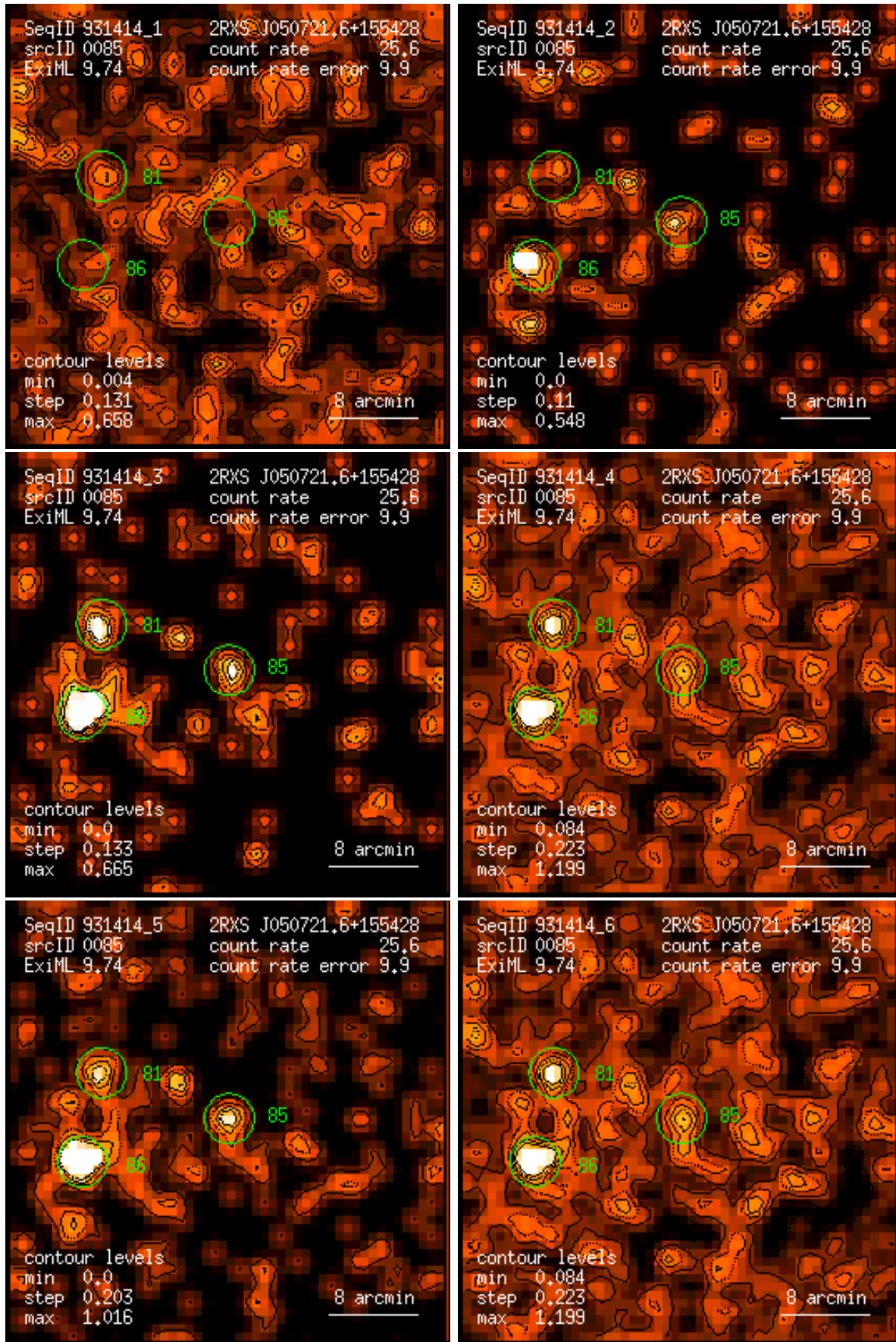
Figure 85: RASS 931414: detection 0085: band rate images, Gaussian filter: (1) PSPC channels 11 – 41, (2) 52 – 90, (3) 91 – 201, (4) 11 – 235, (5) 52 – 201, (6) 11 – 201. Broad band rates in counts/ks. Band rate contour levels in counts/ks/arcmin 2 .
