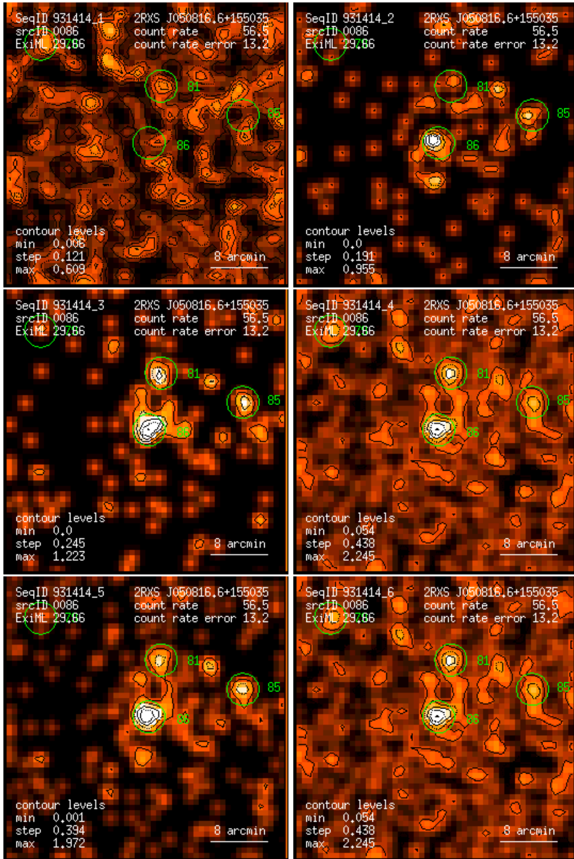
Figure 86: RASS 931414: detection 0086: band rate images, Gaussian filter: (1) PSPC channels 11 – 41, (2) 52 – 90, (3) 91 – 201, (4) 11 – 235, (5) 52 – 201, (6) 11 – 201. Broad band rates in counts/ks. Band rate contour levels in counts/ks/arcmin 2 .
