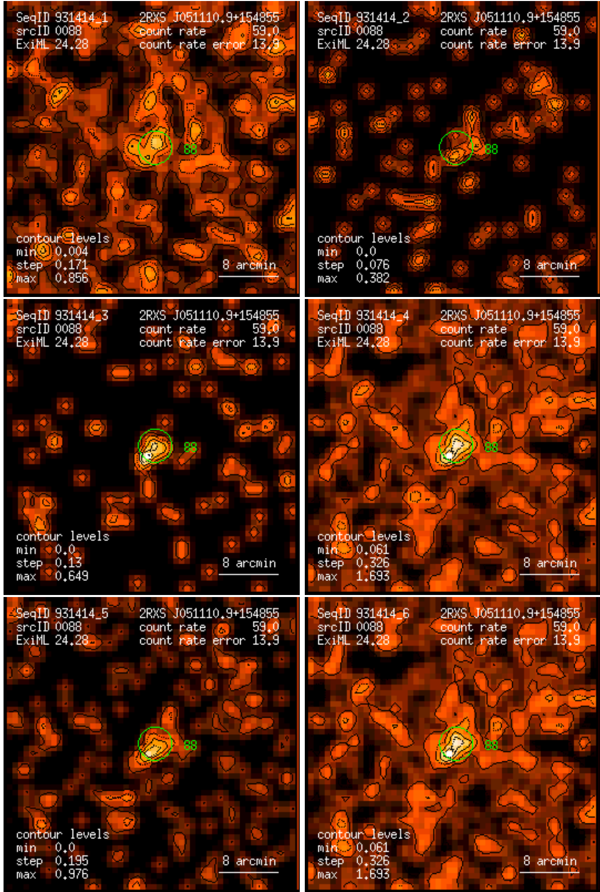
Figure 88: RASS 931414: detection 0088: band rate images, Gaussian filter: (1) PSPC channels 11 – 41, (2) 52 – 90, (3) 91 – 201, (4) 11 – 235, (5) 52 – 201, (6) 11 – 201. Broad band rates in counts/ks. Band rate contour levels in counts/ks/arcmin 2 .
