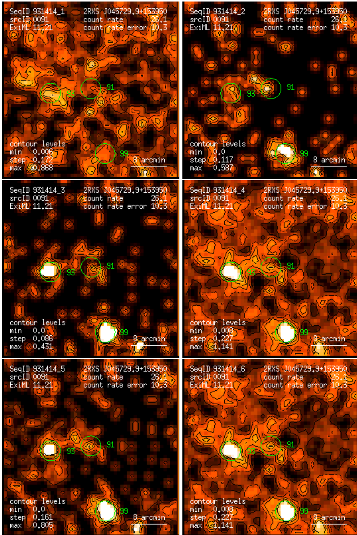
Figure 91: RASS 931414: detection 0091: band rate images, Gaussian filter: (1) PSPC channels 11 – 41, (2) 52 – 90, (3) 91 – 201, (4) 11 – 235, (5) 52 – 201, (6) 11 – 201. Broad band rates in counts/ks. Band rate contour levels in counts/ks/arcmin 2 .
