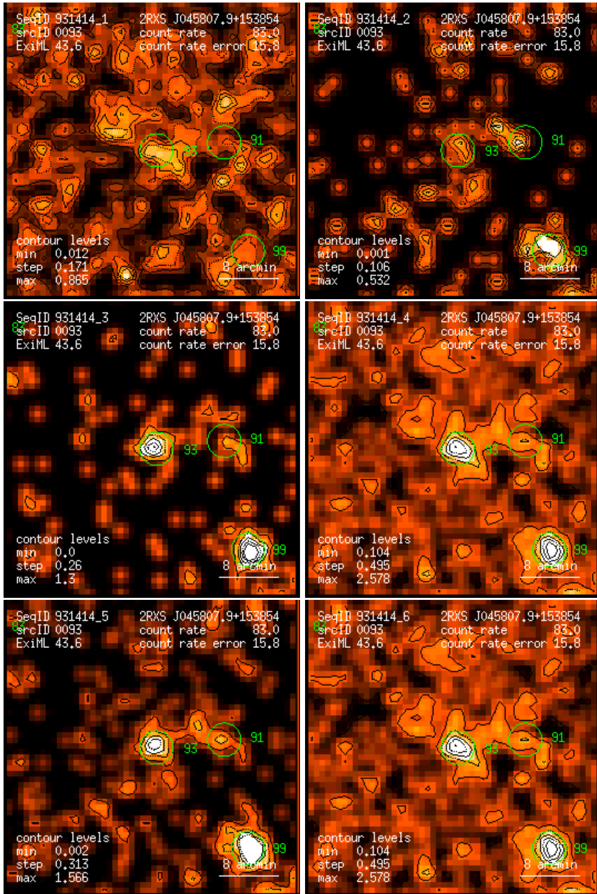
Figure 93: RASS 931414: detection 0093: band rate images, Gaussian filter: (1) PSPC channels 11 – 41, (2) 52 – 90, (3) 91 – 201, (4) 11 – 235, (5) 52 – 201, (6) 11 – 201. Broad band rates in counts/ks. Band rate contour levels in counts/ks/arcmin 2 .
