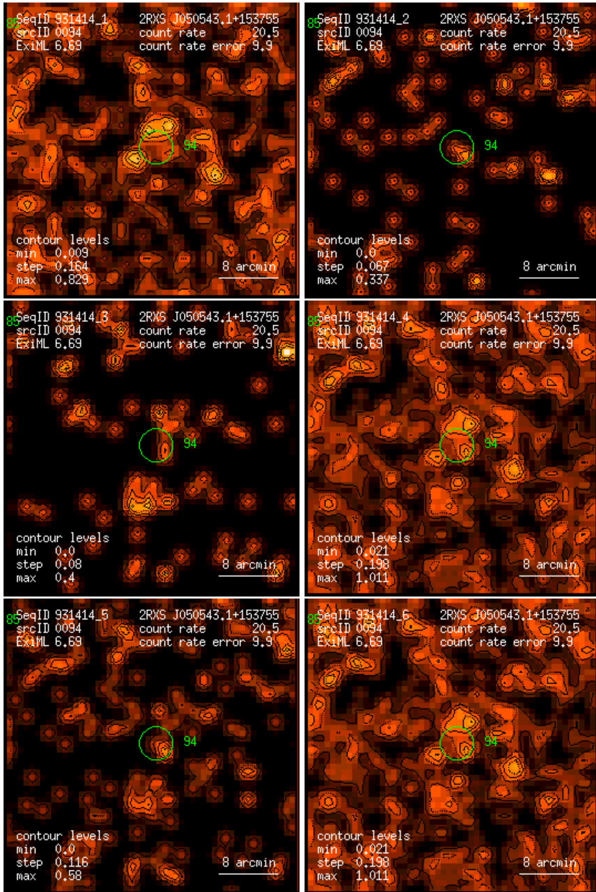
Figure 94: RASS 931414: detection 0094: band rate images, Gaussian filter: (1) PSPC channels 11 – 41, (2) 52 – 90, (3) 91 – 201, (4) 11 – 235, (5) 52 – 201, (6) 11 – 201. Broad band rates in counts/ks. Band rate contour levels in counts/ks/arcmin 2 .
