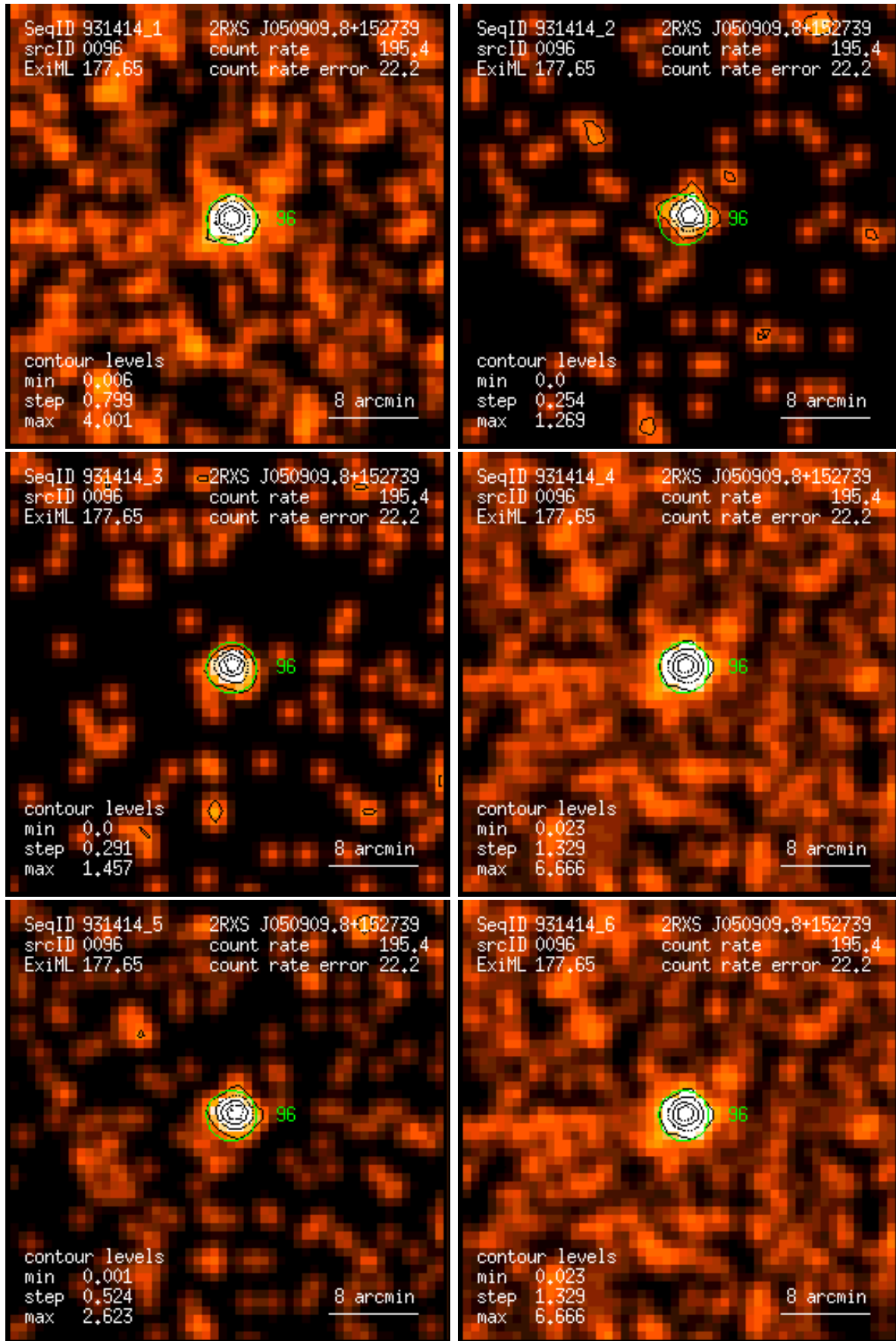
Figure 96: RASS 931414: detection 0096: band rate images, Gaussian filter: (1) PSPC channels 11 – 41, (2) 52 – 90, (3) 91 – 201, (4) 11 – 235, (5) 52 – 201, (6) 11 – 201. Broad band rates in counts/ks. Band rate contour levels in counts/ks/arcmin 2 .
