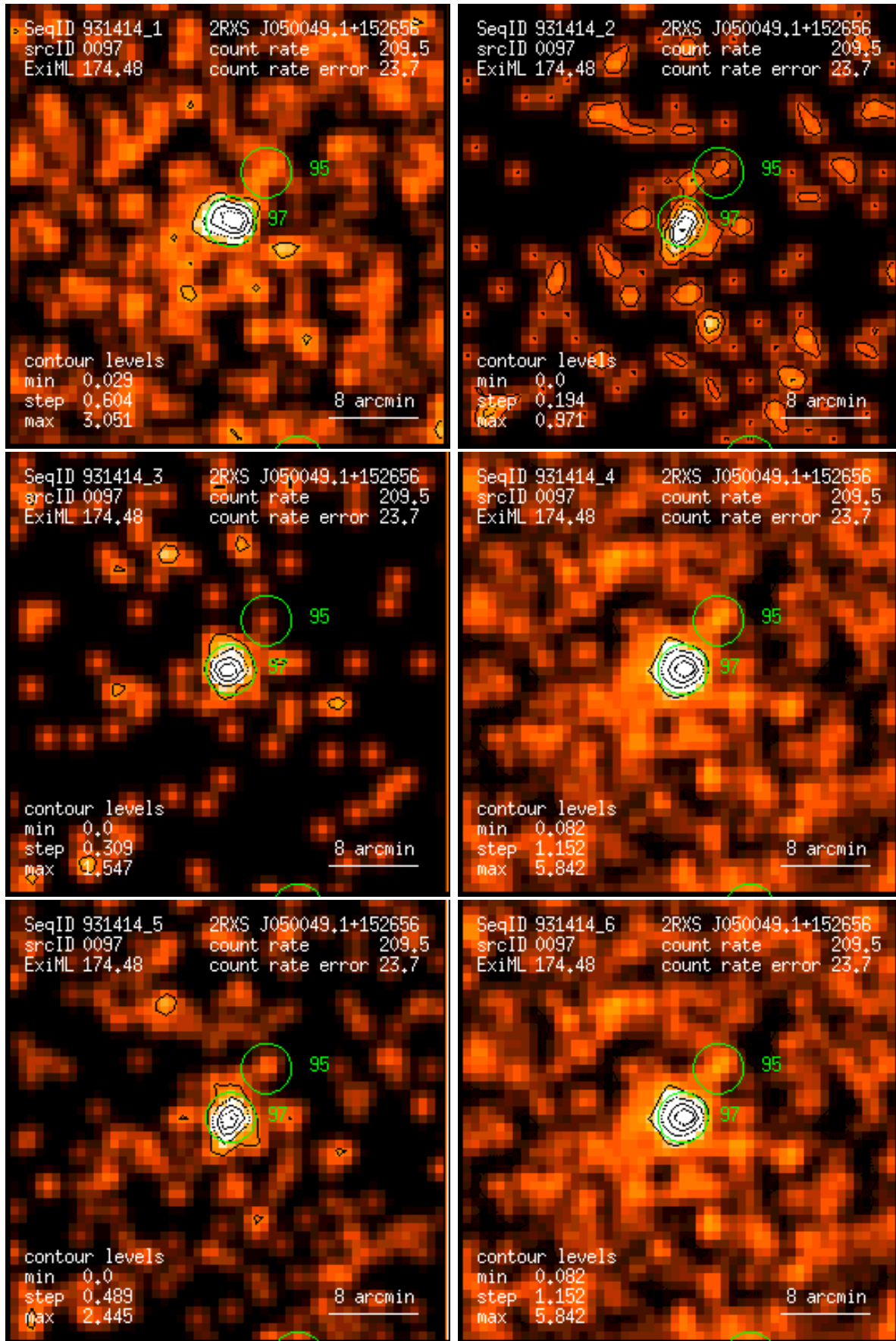
Figure 97: RASS 931414: detection 0097: band rate images, Gaussian filter: (1) PSPC channels 11 – 41, (2) 52 – 90, (3) 91 – 201, (4) 11 – 235, (5) 52 – 201, (6) 11 – 201. Broad band rates in counts/ks. Band rate contour levels in counts/ks/arcmin 2 .
