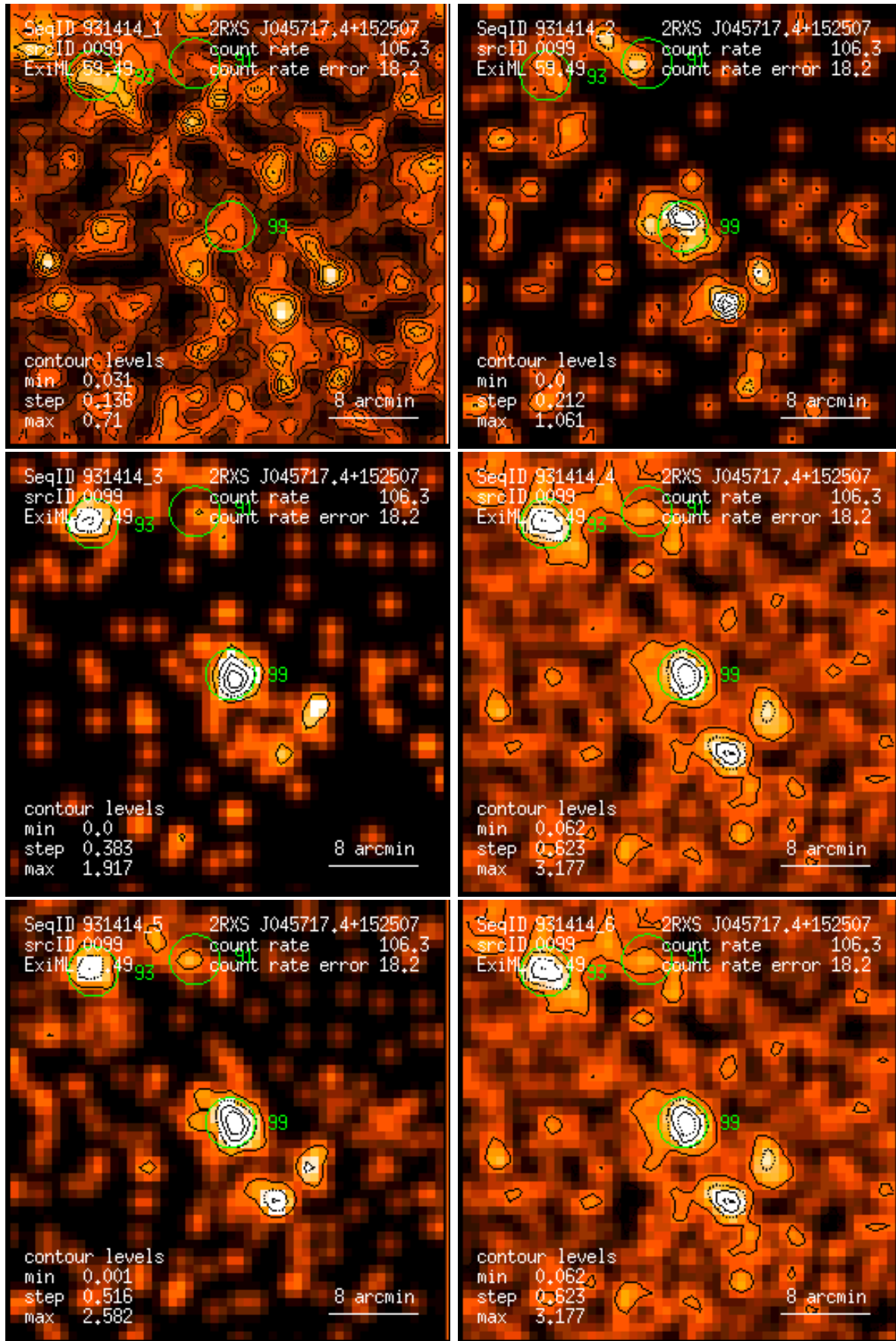
Figure 99: RASS 931414: detection 0099: band rate images, Gaussian filter: (1) PSPC channels 11 – 41, (2) 52 – 90, (3) 91 – 201, (4) 11 – 235, (5) 52 – 201, (6) 11 – 201. Broad band rates in counts/ks. Band rate contour levels in counts/ks/arcmin 2 .
