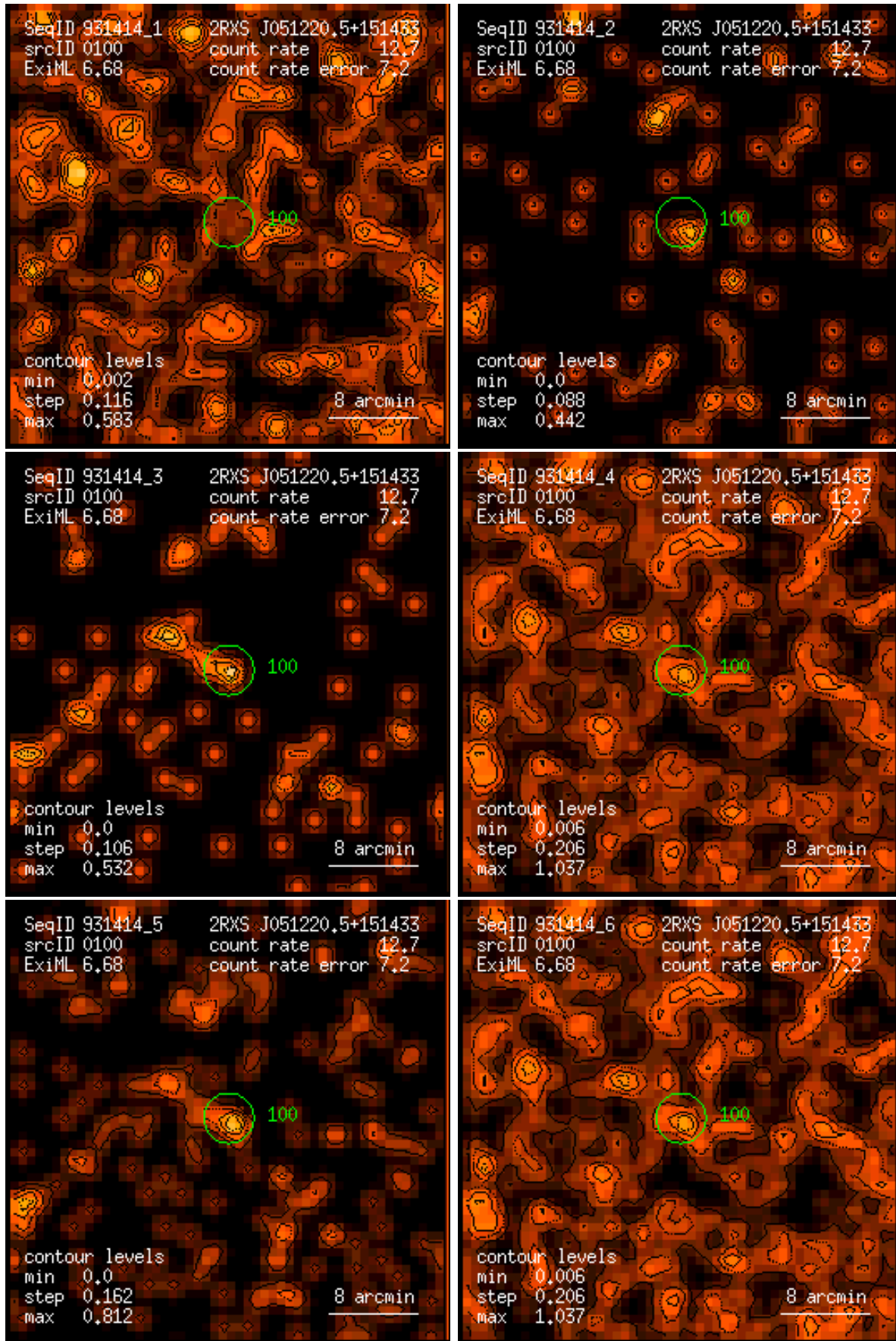
Figure 100: RASS 931414: detection 0100: band rate images, Gaussian filter: (1) PSPC channels 11 – 41, (2) 52 – 90, (3) 91 – 201, (4) 11 – 235, (5) 52 – 201, (6) 11 – 201. Broad band rates in counts/ks. Band rate contour levels in counts/ks/arcmin 2 .
