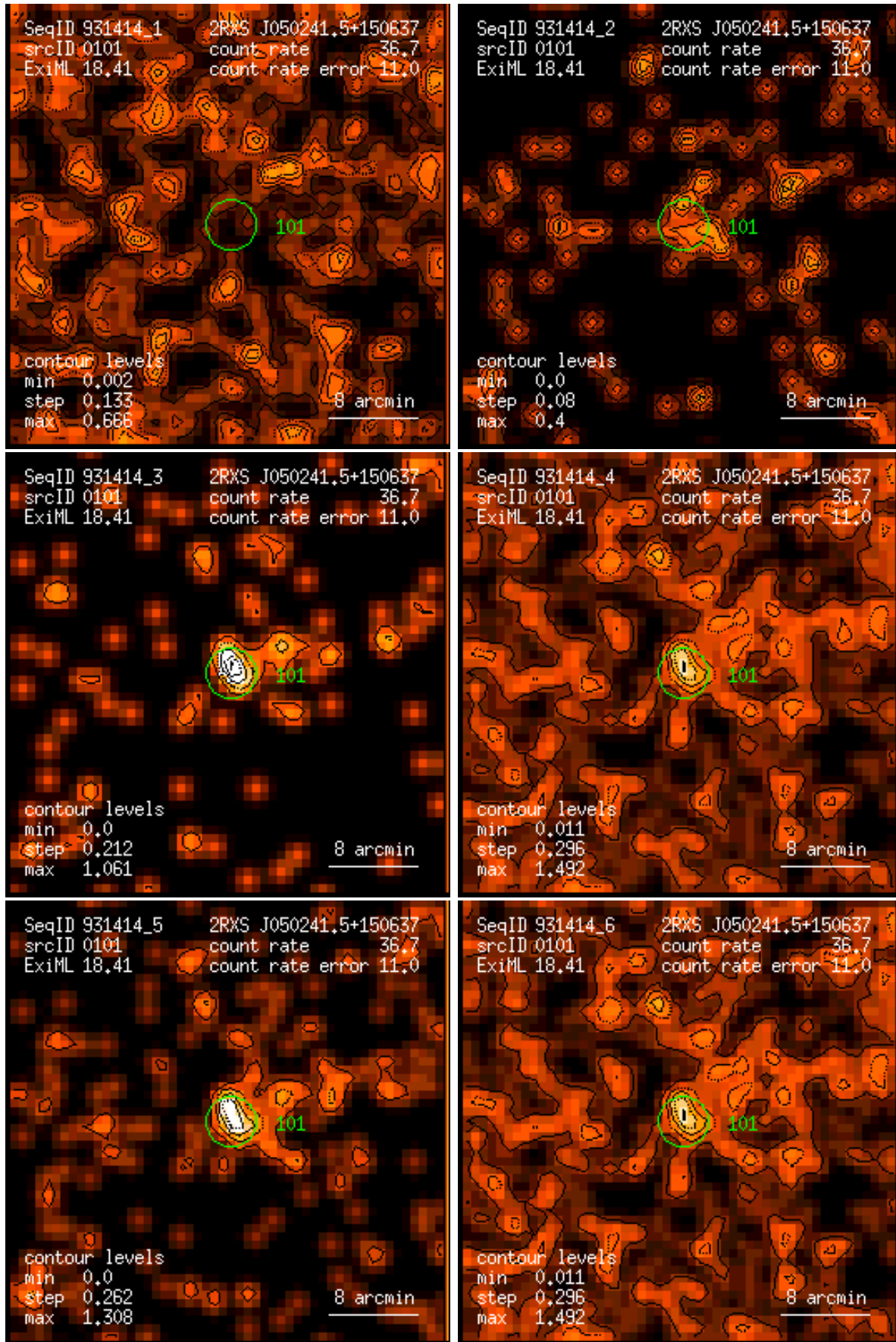
Figure 101: RASS 931414: detection 0101: band rate images, Gaussian filter: (1) PSPC channels 11 – 41, (2) 52 – 90, (3) 91 – 201, (4) 11 – 235, (5) 52 – 201, (6) 11 – 201. Broad band rates in counts/ks. Band rate contour levels in counts/ks/arcmin 2 .
