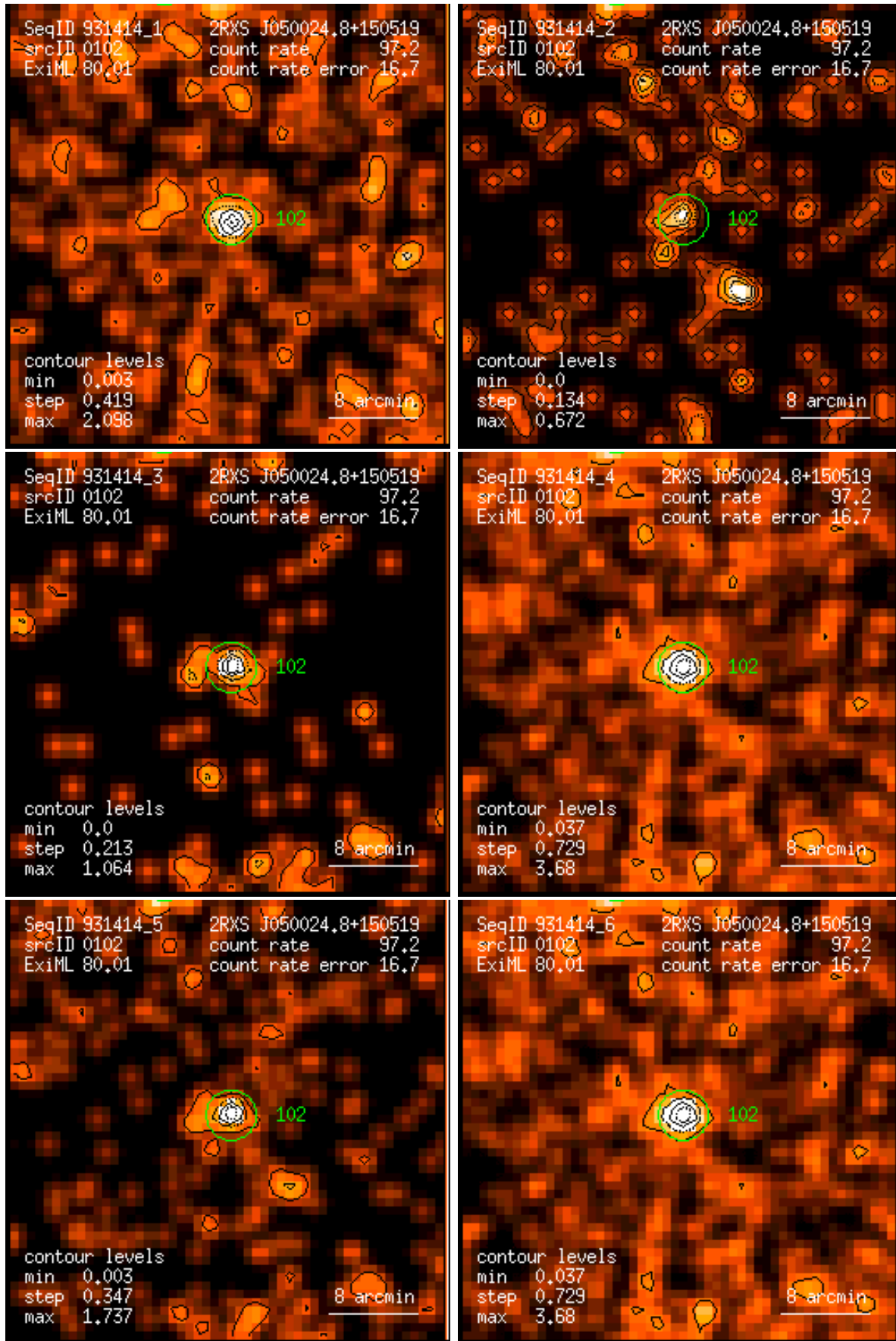
Figure 102: RASS 931414: detection 0102: band rate images, Gaussian filter: (1) PSPC channels 11 – 41, (2) 52 – 90, (3) 91 – 201, (4) 11 – 235, (5) 52 – 201, (6) 11 – 201. Broad band rates in counts/ks. Band rate contour levels in counts/ks/arcmin 2 .
