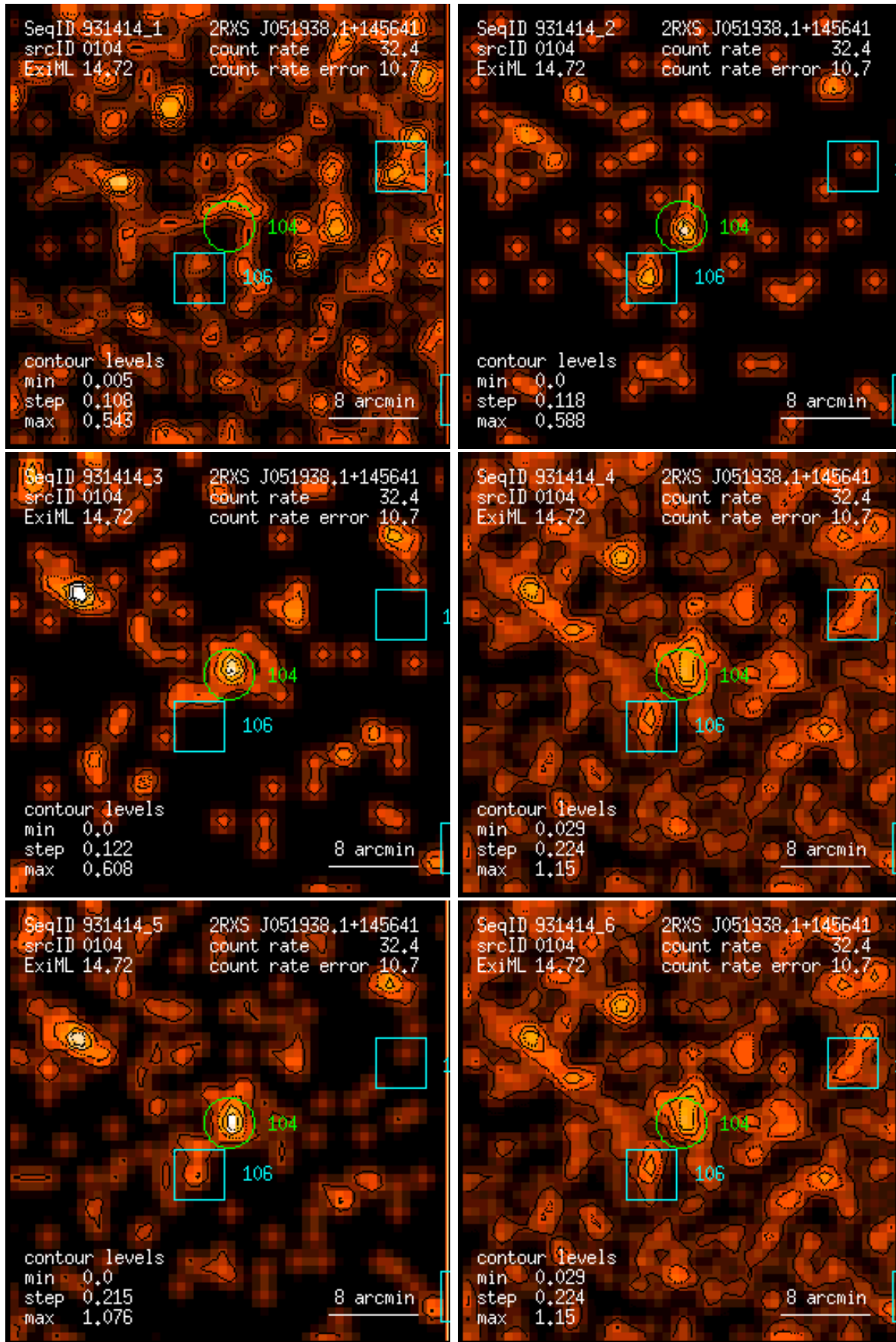
Figure 104: RASS 931414: detection 0104: band rate images, Gaussian filter: (1) PSPC channels 11 – 41, (2) 52 – 90, (3) 91 – 201, (4) 11 – 235, (5) 52 – 201, (6) 11 – 201. Broad band rates in counts/ks. Band rate contour levels in counts/ks/arcmin 2 .
