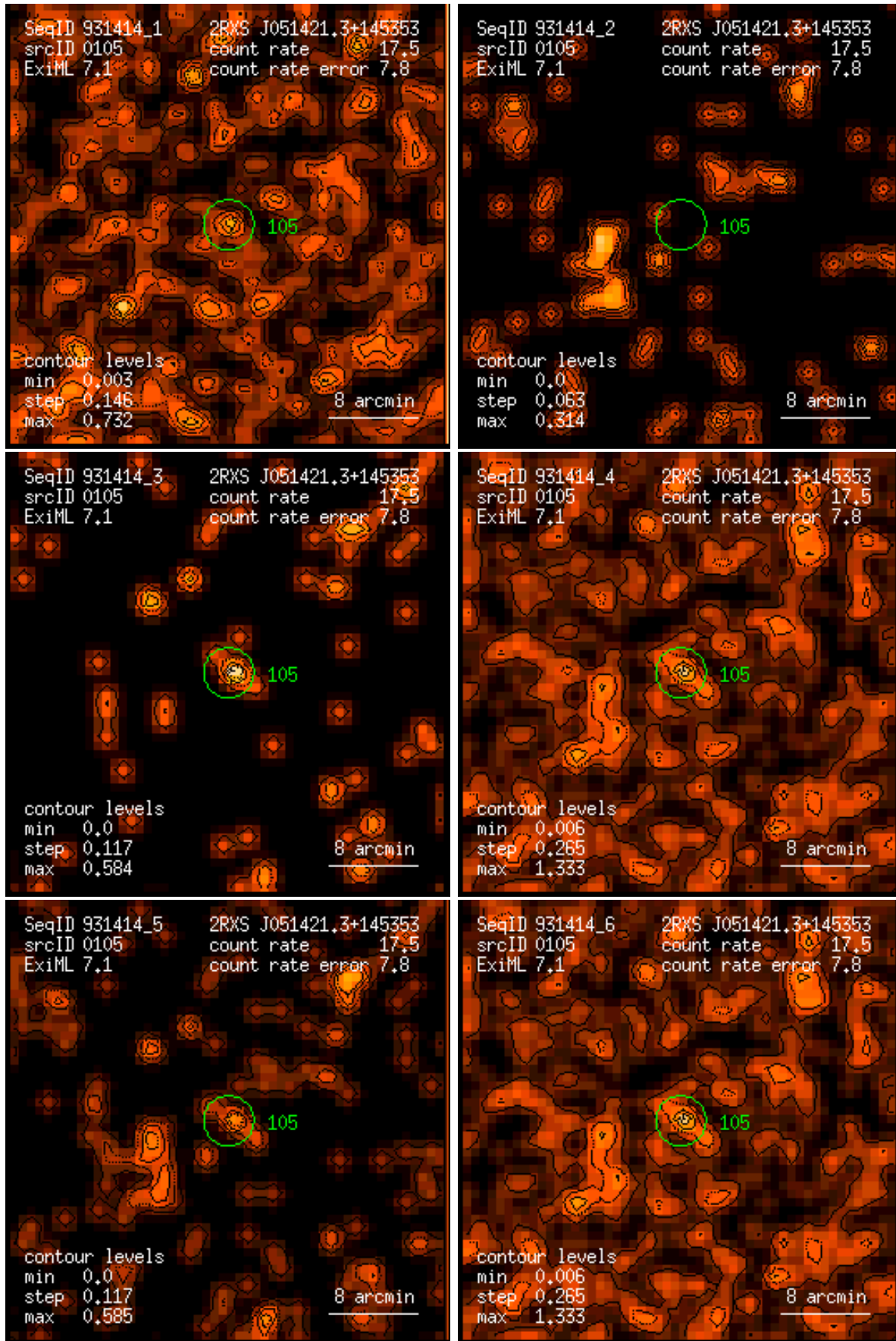
Figure 105: RASS 931414: detection 0105: band rate images, Gaussian filter: (1) PSPC channels 11 – 41, (2) 52 – 90, (3) 91 – 201, (4) 11 – 235, (5) 52 – 201, (6) 11 – 201. Broad band rates in counts/ks. Band rate contour levels in counts/ks/arcmin 2 .
