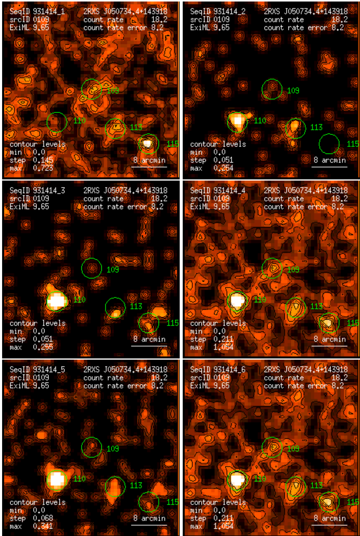
Figure 109: RASS 931414: detection 0109: band rate images, Gaussian filter: (1) PSPC channels 11 – 41, (2) 52 – 90, (3) 91 – 201, (4) 11 – 235, (5) 52 – 201, (6) 11 – 201. Broad band rates in counts/ks. Band rate contour levels in counts/ks/arcmin 2 .
