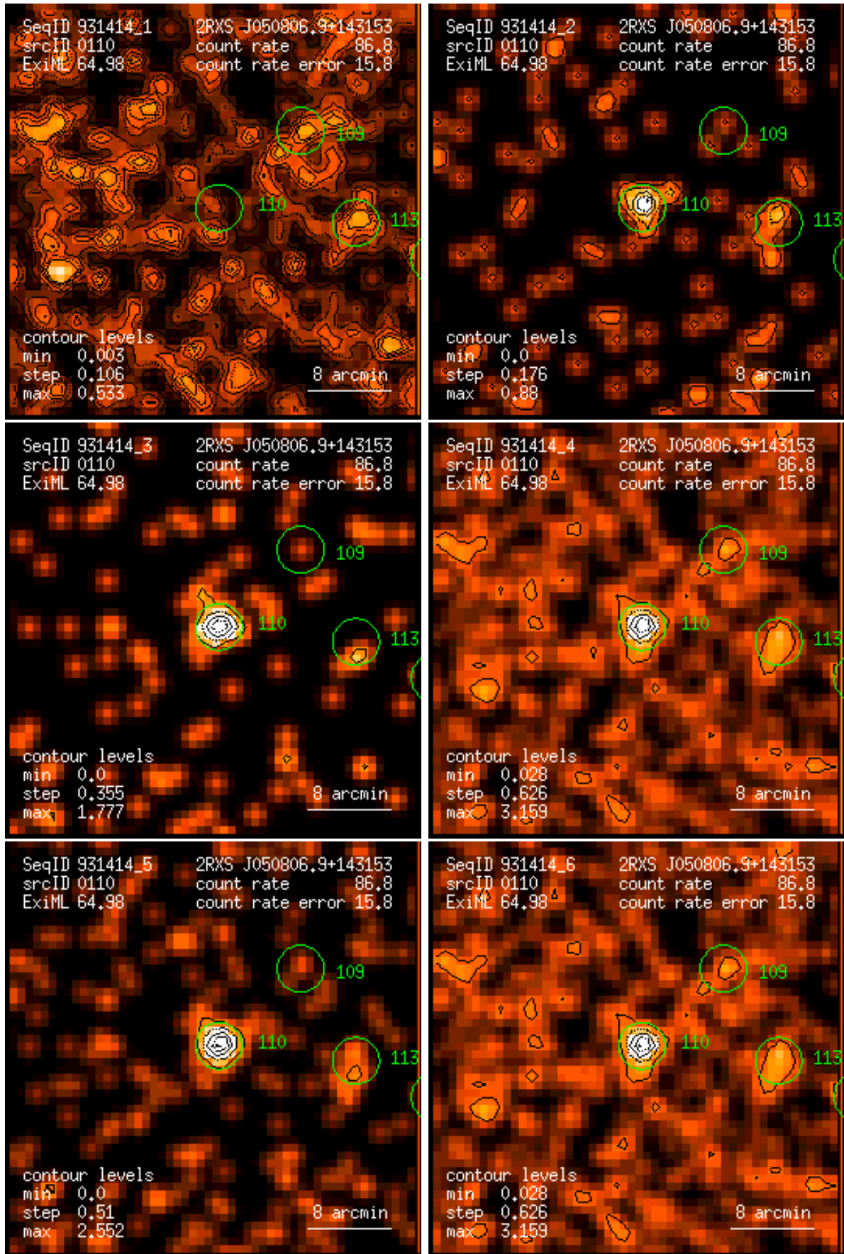
Figure 110: RASS 931414: detection 0110: band rate images, Gaussian filter: (1) PSPC channels 11 – 41, (2) 52 – 90, (3) 91 – 201, (4) 11 – 235, (5) 52 – 201, (6) 11 – 201. Broad band rates in counts/ks. Band rate contour levels in counts/ks/arcmin 2 .
