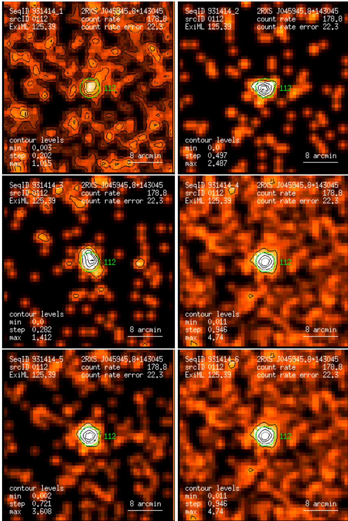
Figure 112: RASS 931414: detection 0112: band rate images, Gaussian filter: (1) PSPC channels 11 – 41, (2) 52 – 90, (3) 91 – 201, (4) 11 – 235, (5) 52 – 201, (6) 11 – 201. Broad band rates in counts/ks. Band rate contour levels in counts/ks/arcmin 2 .
