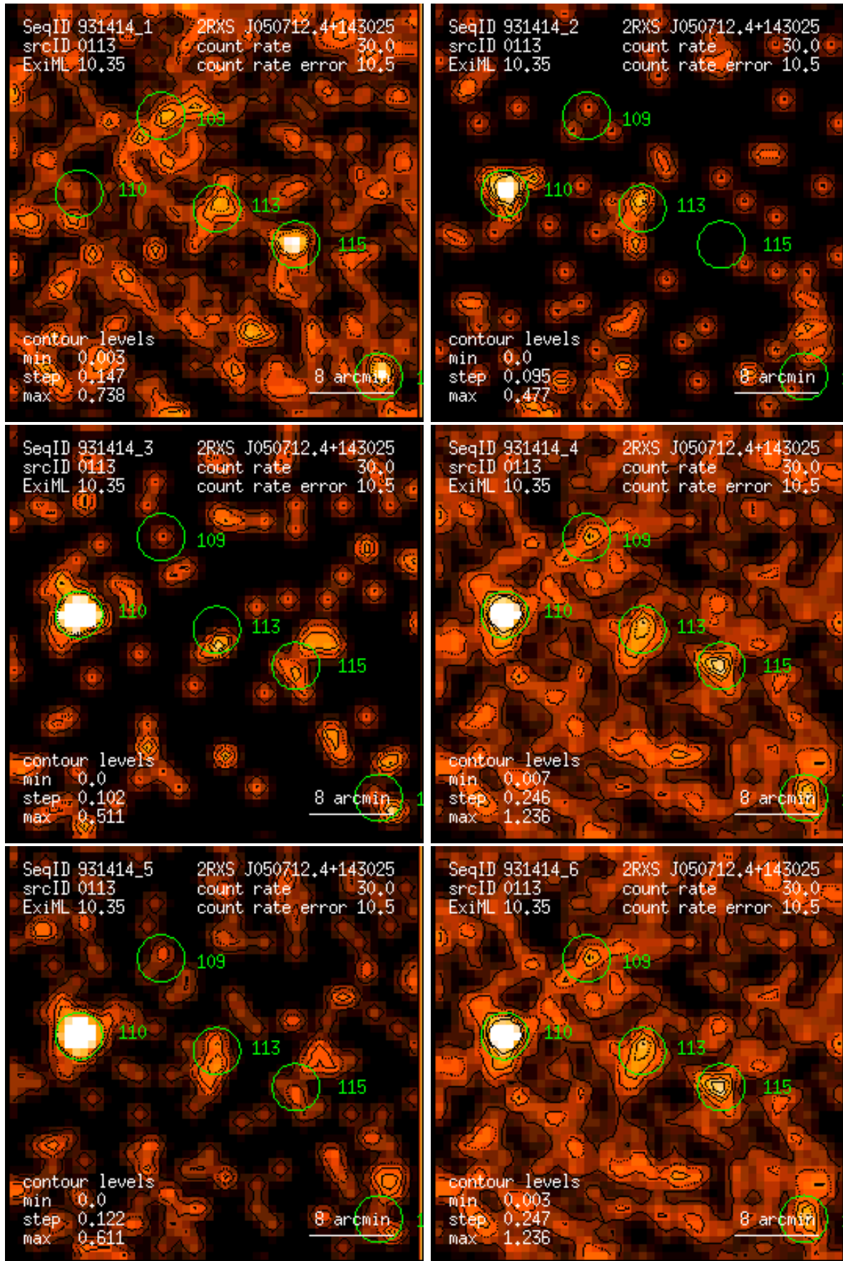
Figure 113: RASS 931414: detection 0113: band rate images, Gaussian filter: (1) PSPC channels 11 – 41, (2) 52 – 90, (3) 91 – 201, (4) 11 – 235, (5) 52 – 201, (6) 11 – 201. Broad band rates in counts/ks. Band rate contour levels in counts/ks/arcmin 2 .
