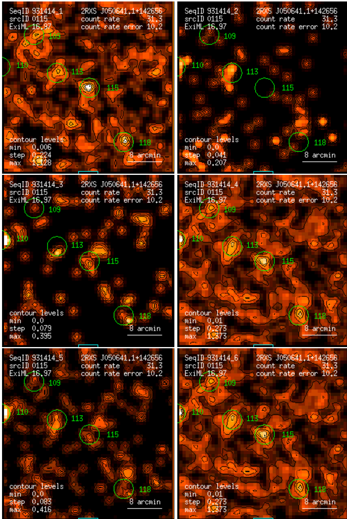
Figure 115: RASS 931414: detection 0115: band rate images, Gaussian filter: (1) PSPC channels 11 – 41, (2) 52 – 90, (3) 91 – 201, (4) 11 – 235, (5) 52 – 201, (6) 11 – 201. Broad band rates in counts/ks. Band rate contour levels in counts/ks/arcmin 2 .
