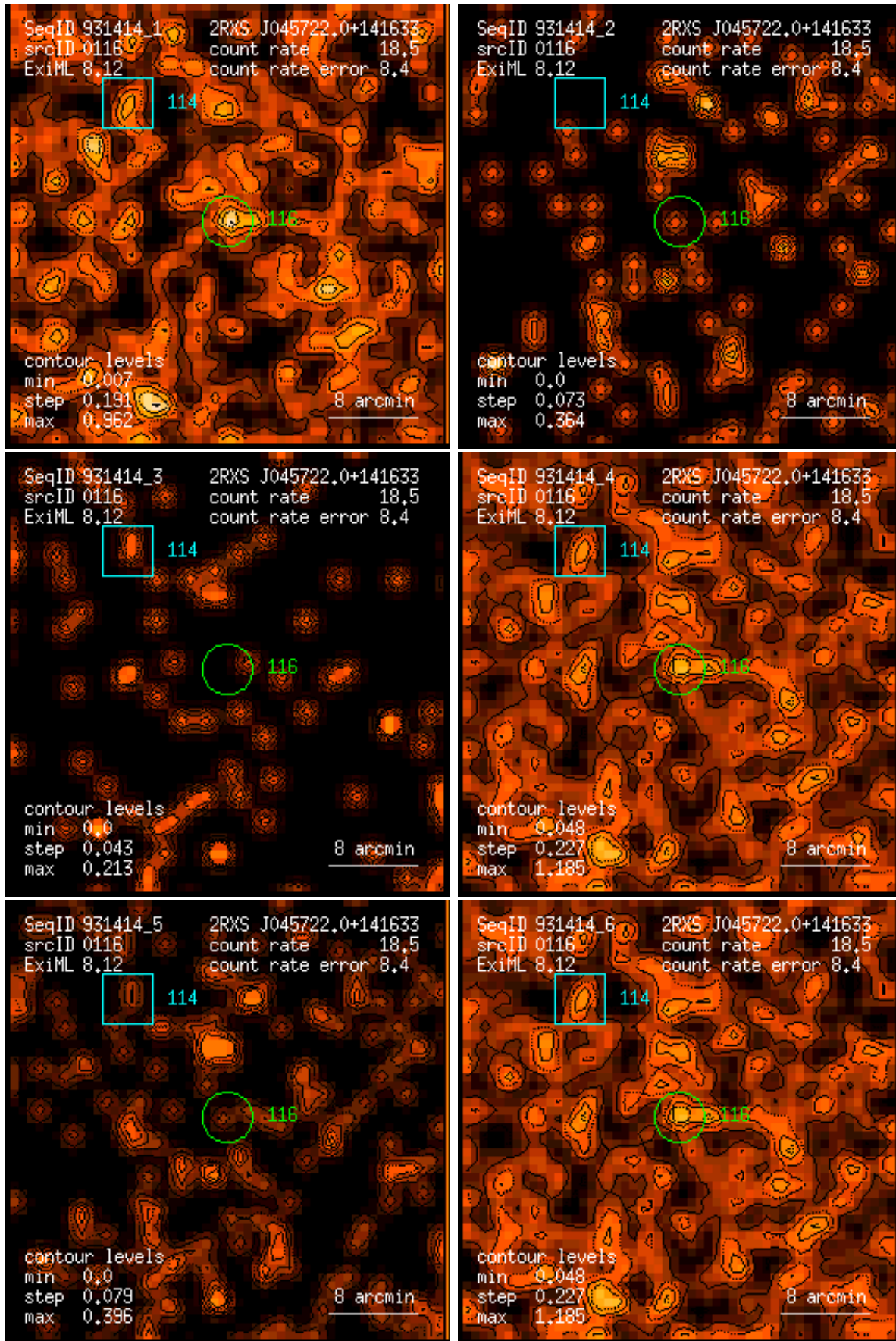
Figure 116: RASS 931414: detection 0116: band rate images, Gaussian filter: (1) PSPC channels 11 – 41, (2) 52 – 90, (3) 91 – 201, (4) 11 – 235, (5) 52 – 201, (6) 11 – 201. Broad band rates in counts/ks. Band rate contour levels in counts/ks/arcmin 2 .
