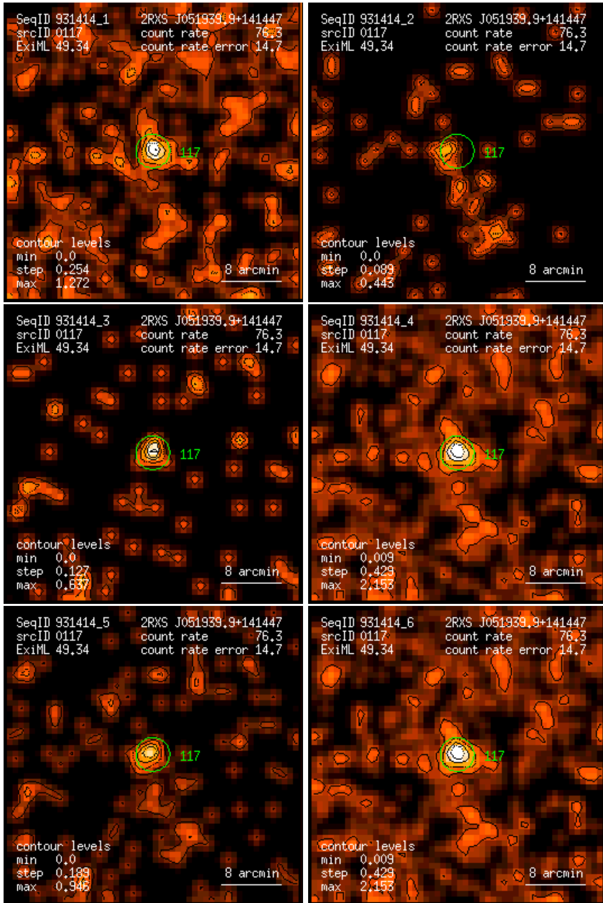
Figure 117: RASS 931414: detection 0117: band rate images, Gaussian filter: (1) PSPC channels 11 – 41, (2) 52 – 90, (3) 91 – 201, (4) 11 – 235, (5) 52 – 201, (6) 11 – 201. Broad band rates in counts/ks. Band rate contour levels in counts/ks/arcmin 2 .
