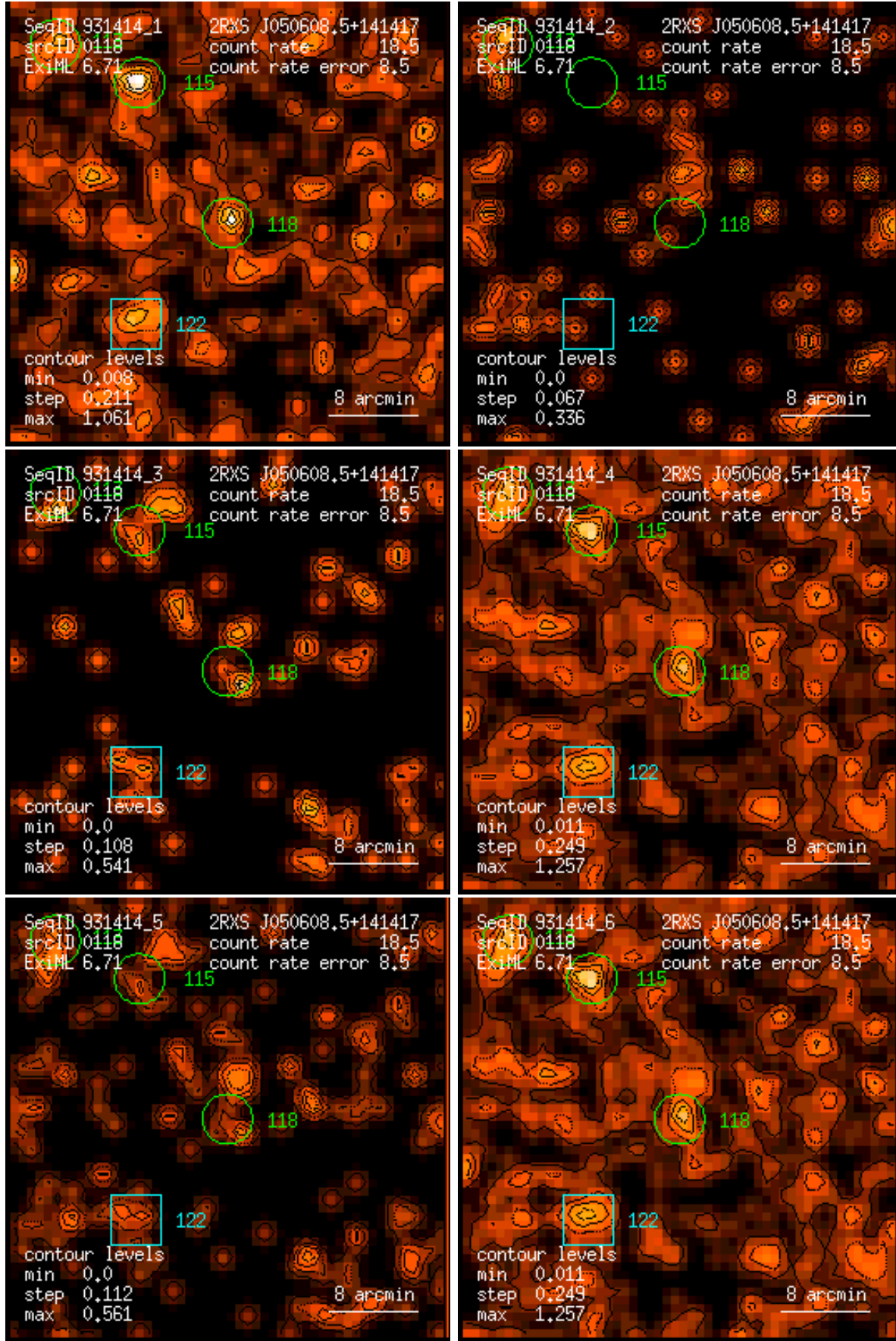
Figure 118: RASS 931414: detection 0118: band rate images, Gaussian filter: (1) PSPC channels 11 – 41, (2) 52 – 90, (3) 91 – 201, (4) 11 – 235, (5) 52 – 201, (6) 11 – 201. Broad band rates in counts/ks. Band rate contour levels in counts/ks/arcmin 2 .
