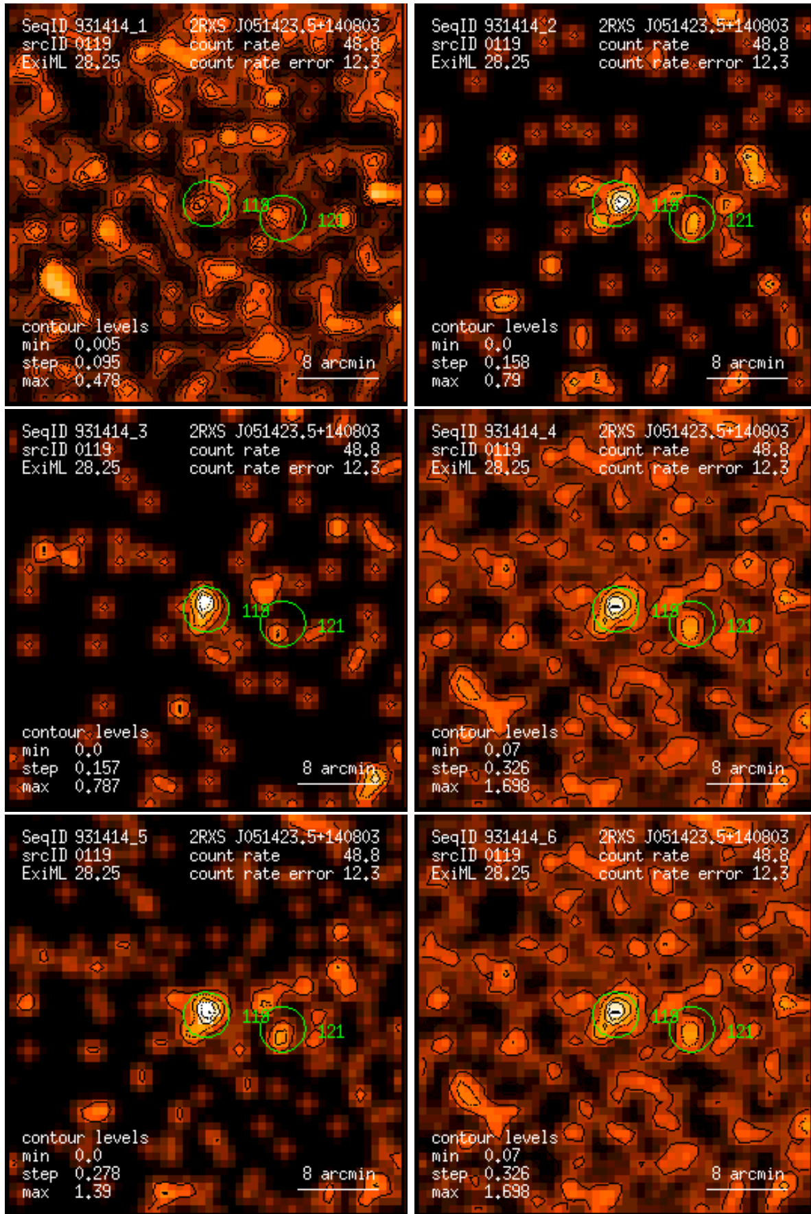
Figure 119: RASS 931414: detection 0119: band rate images, Gaussian filter: (1) PSPC channels 11 – 41, (2) 52 – 90, (3) 91 – 201, (4) 11 – 235, (5) 52 – 201, (6) 11 – 201. Broad band rates in counts/ks. Band rate contour levels in counts/ks/arcmin 2 .
