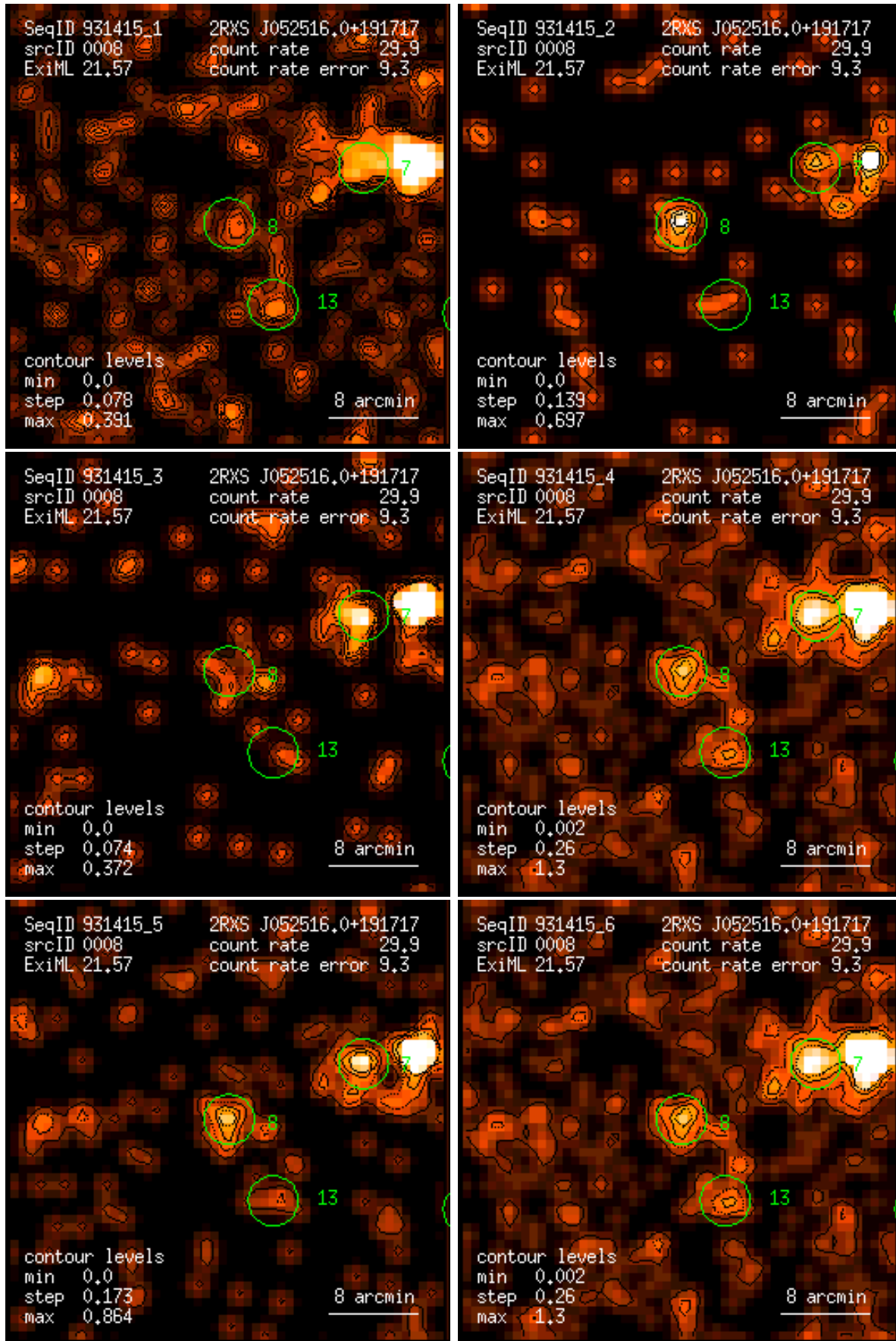
Figure 8: RASS 931415: detection 0008: band rate images, Gaussian filter: (1) PSPC channels 11 – 41, (2) 52 – 90, (3) 91 – 201, (4) 11 – 235, (5) 52 – 201, (6) 11 – 201. Broad band rates in counts/ks. Band rate contour levels in counts/ks/arcmin 2 .
