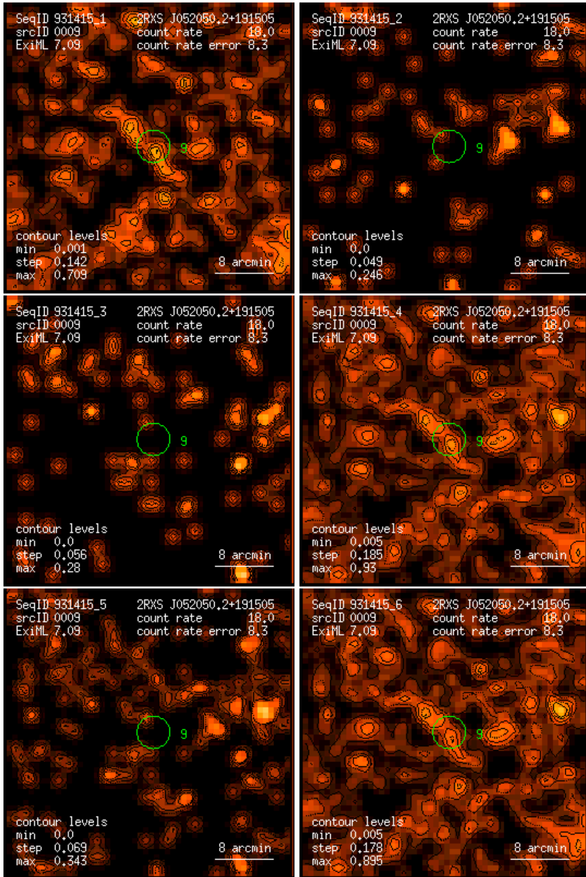
Figure 9: RASS 931415: detection 0009: band rate images, Gaussian filter: (1) PSPC channels 11 – 41, (2) 52 – 90, (3) 91 – 201, (4) 11 – 235, (5) 52 – 201, (6) 11 – 201. Broad band rates in counts/ks. Band rate contour levels in counts/ks/arcmin 2 .
