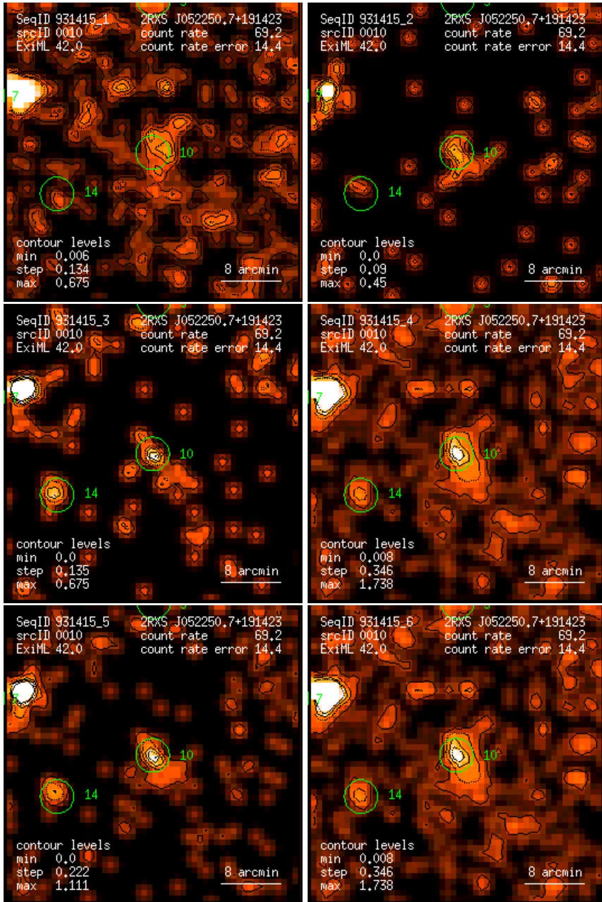
Figure 10: RASS 931415: detection 0010: band rate images, Gaussian filter: (1) PSPC channels 11 – 41, (2) 52 – 90, (3) 91 – 201, (4) 11 – 235, (5) 52 – 201, (6) 11 – 201. Broad band rates in counts/ks. Band rate contour levels in counts/ks/arcmin 2 .
