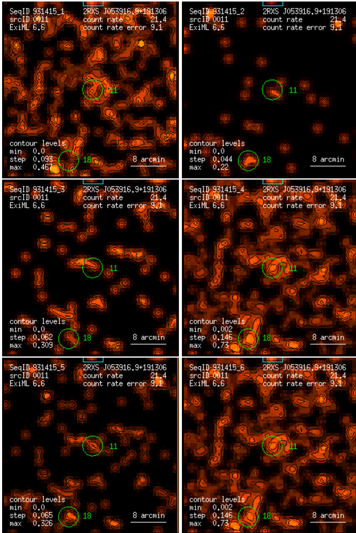
Figure 11: RASS 931415: detection 0011: band rate images, Gaussian filter: (1) PSPC channels 11 – 41, (2) 52 – 90, (3) 91 – 201, (4) 11 – 235, (5) 52 – 201, (6) 11 – 201. Broad band rates in counts/ks. Band rate contour levels in counts/ks/arcmin 2 .
