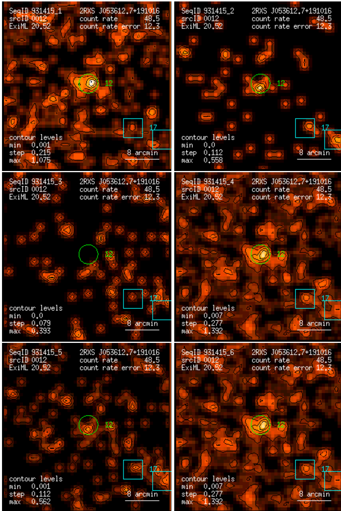
Figure 12: RASS 931415: detection 0012: band rate images, Gaussian filter: (1) PSPC channels 11 – 41, (2) 52 – 90, (3) 91 – 201, (4) 11 – 235, (5) 52 – 201, (6) 11 – 201. Broad band rates in counts/ks. Band rate contour levels in counts/ks/arcmin 2 .
