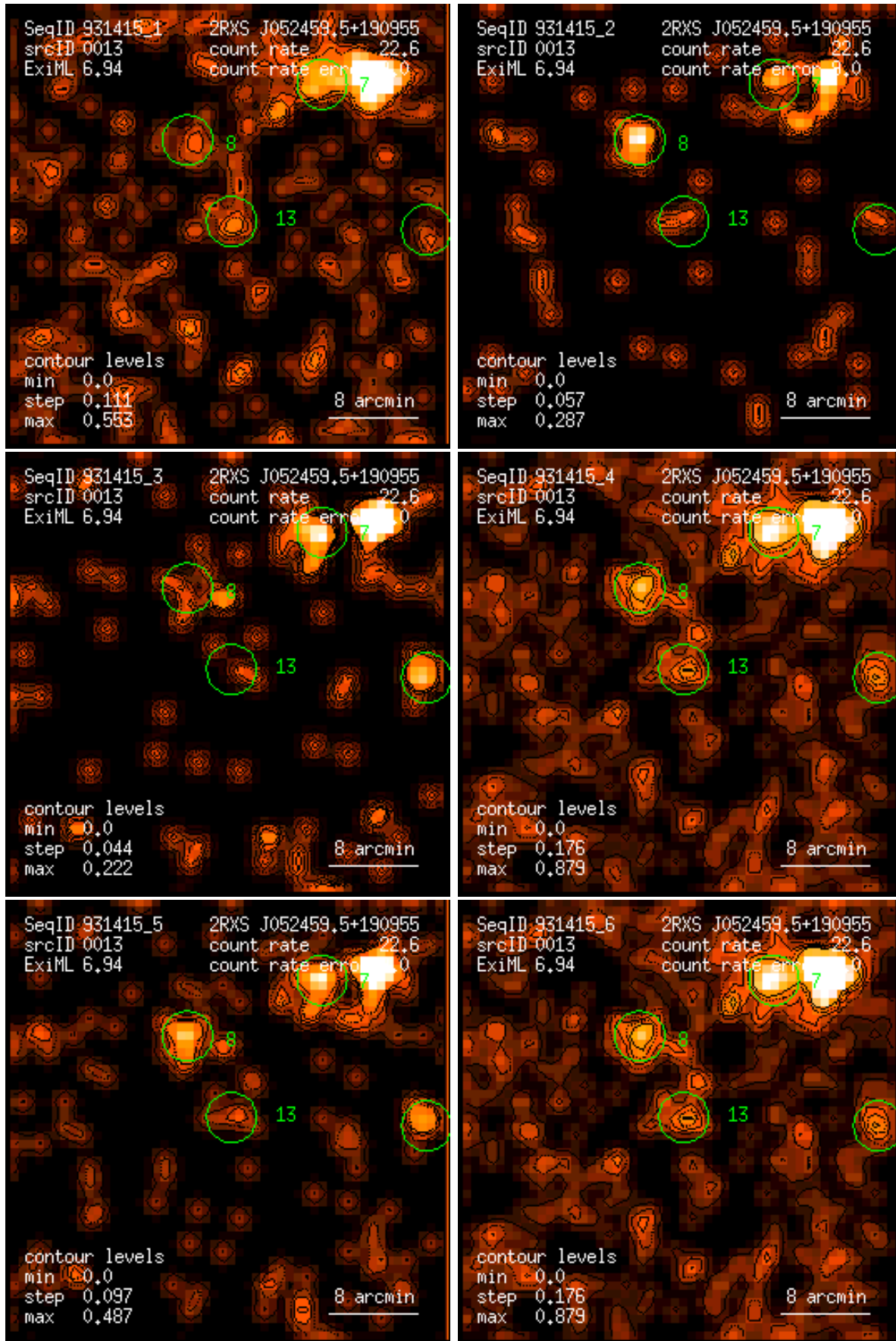
Figure 13: RASS 931415: detection 0013: band rate images, Gaussian filter: (1) PSPC channels 11 – 41, (2) 52 – 90, (3) 91 – 201, (4) 11 – 235, (5) 52 – 201, (6) 11 – 201. Broad band rates in counts/ks. Band rate contour levels in counts/ks/arcmin 2 .
